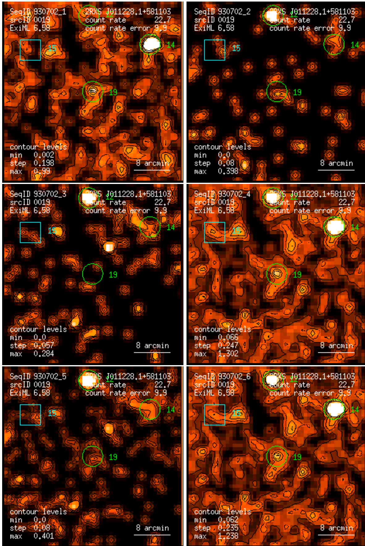
Figure 19: RASS 930702: detection 0019: band rate images, Gaussian filter: (1) PSPC channels 11 – 41, (2) 52 – 90, (3) 91 – 201, (4) 11 – 235, (5) 52 – 201, (6) 11 – 201. Broad band rates in counts/ks. Band rate contour levels in counts/ks/arcmin 2 .
