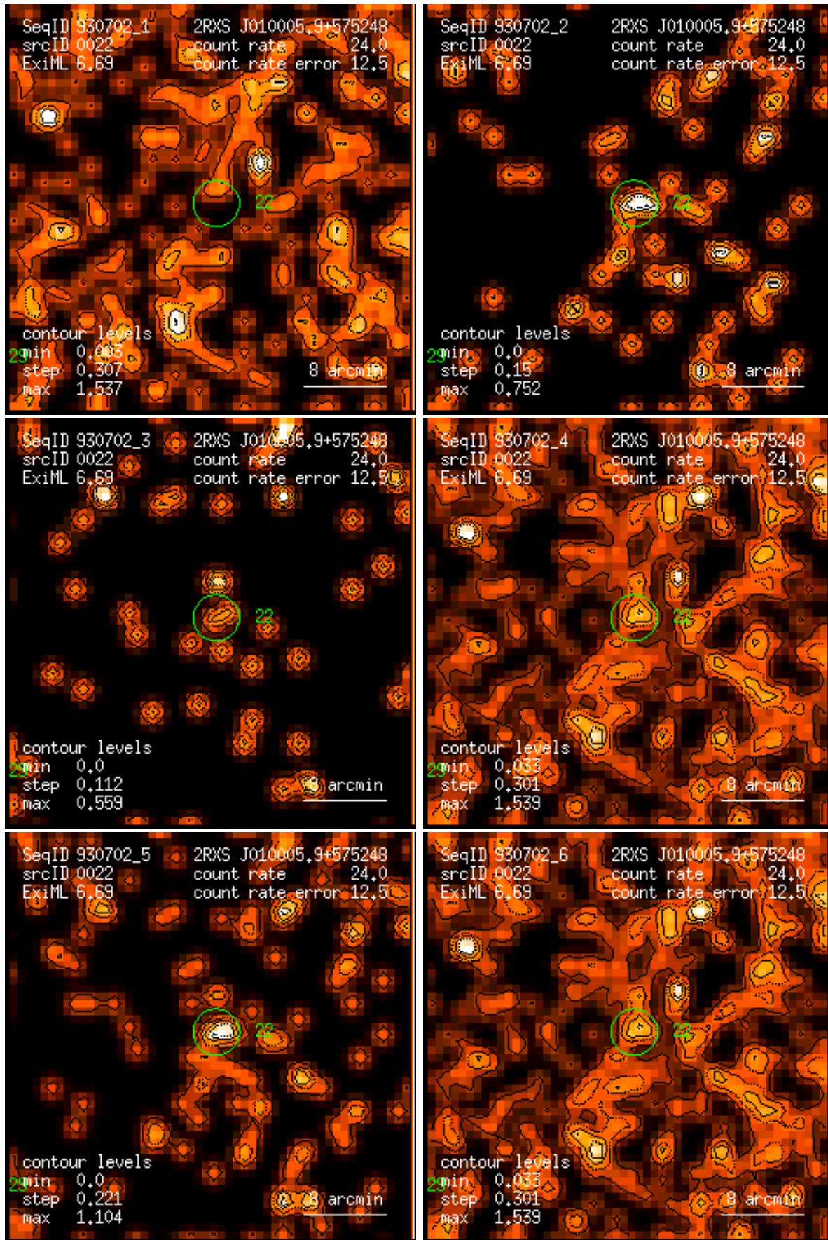
Figure 22: RASS 930702: detection 0022: band rate images, Gaussian filter: (1) PSPC channels 11 – 41, (2) 52 – 90, (3) 91 – 201, (4) 11 – 235, (5) 52 – 201, (6) 11 – 201. Broad band rates in counts/ks. Band rate contour levels in counts/ks/arcmin 2 .
