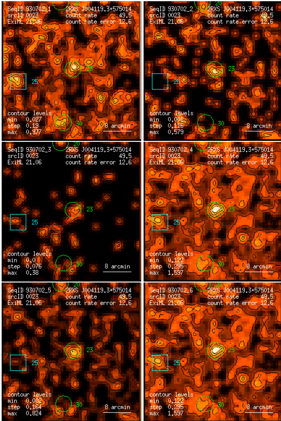
Figure 23: RASS 930702: detection 0023: band rate images, Gaussian filter: (1) PSPC channels 11 – 41, (2) 52 – 90, (3) 91 – 201, (4) 11 – 235, (5) 52 – 201, (6) 11 – 201. Broad band rates in counts/ks. Band rate contour levels in counts/ks/arcmin 2 .
