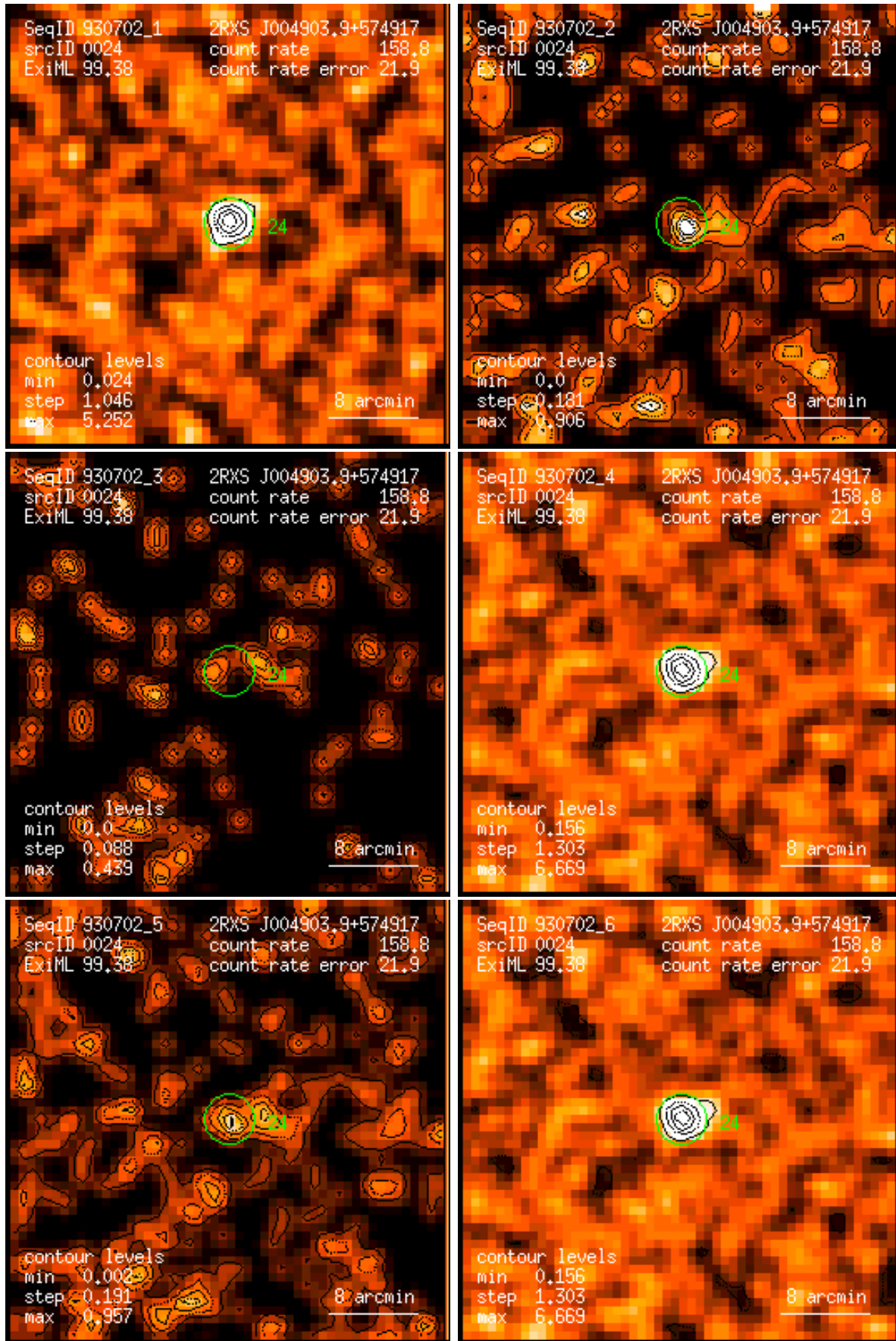
Figure 24: RASS 930702: detection 0024: band rate images, Gaussian filter: (1) PSPC channels 11 – 41, (2) 52 – 90, (3) 91 – 201, (4) 11 – 235, (5) 52 – 201, (6) 11 – 201. Broad band rates in counts/ks. Band rate contour levels in counts/ks/arcmin 2 .
