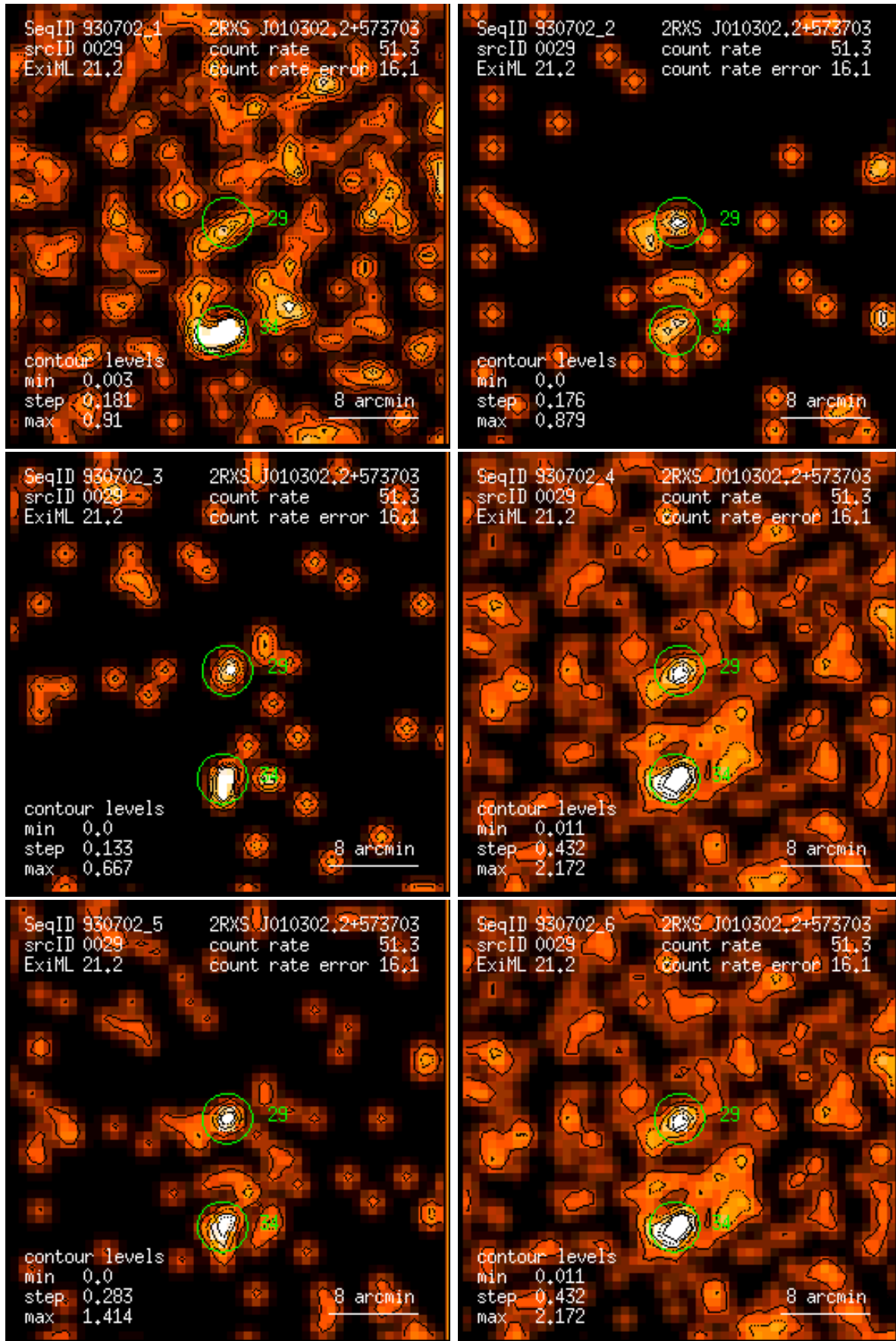
Figure 29: RASS 930702: detection 0029: band rate images, Gaussian filter: (1) PSPC channels 11 – 41, (2) 52 – 90, (3) 91 – 201, (4) 11 – 235, (5) 52 – 201, (6) 11 – 201. Broad band rates in counts/ks. Band rate contour levels in counts/ks/arcmin 2 .
