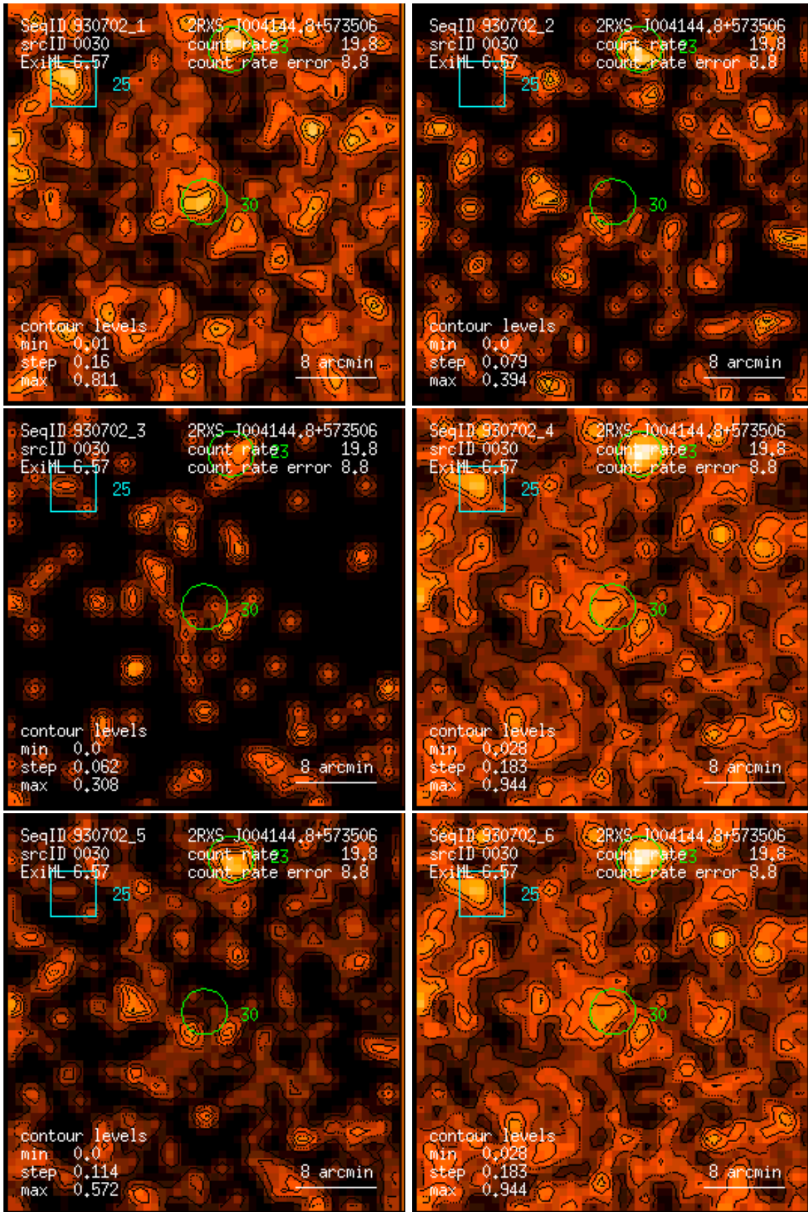
Figure 30: RASS 930702: detection 0030: band rate images, Gaussian filter: (1) PSPC channels 11 – 41, (2) 52 – 90, (3) 91 – 201, (4) 11 – 235, (5) 52 – 201, (6) 11 – 201. Broad band rates in counts/ks. Band rate contour levels in counts/ks/arcmin 2 .
