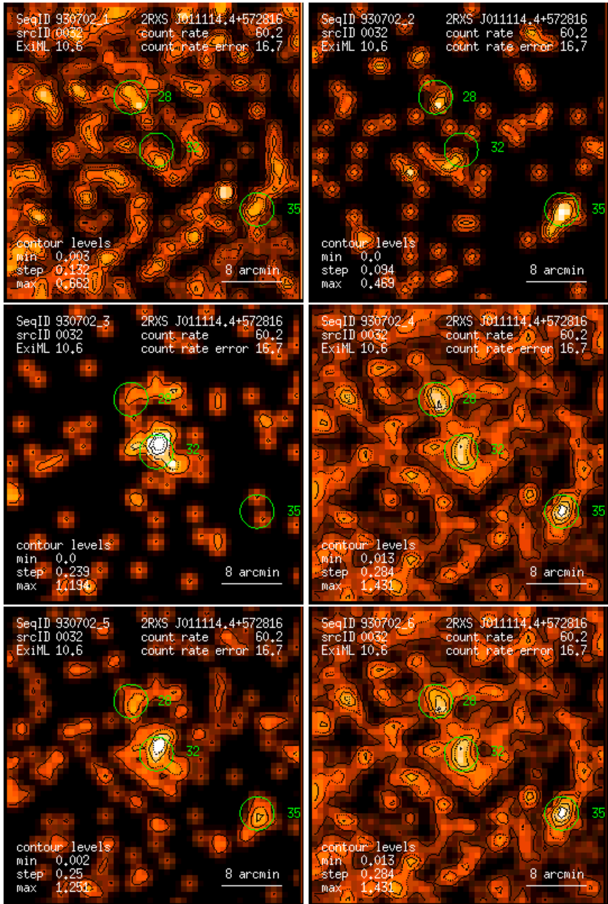
Figure 32: RASS 930702: detection 0032: band rate images, Gaussian filter: (1) PSPC channels 11 – 41, (2) 52 – 90, (3) 91 – 201, (4) 11 – 235, (5) 52 – 201, (6) 11 – 201. Broad band rates in counts/ks. Band rate contour levels in counts/ks/arcmin 2 .
