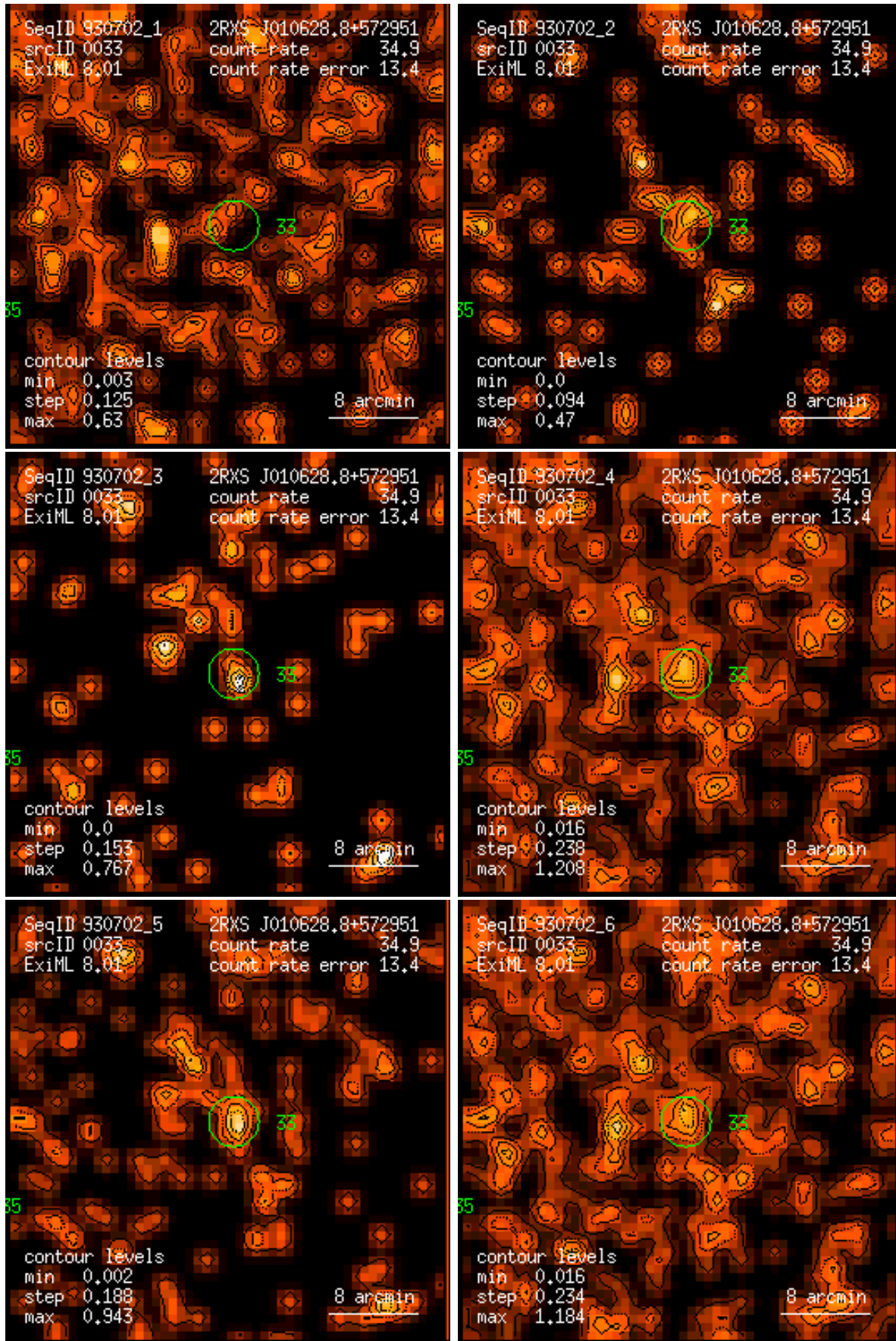
Figure 33: RASS 930702: detection 0033: band rate images, Gaussian filter: (1) PSPC channels 11 – 41, (2) 52 – 90, (3) 91 – 201, (4) 11 – 235, (5) 52 – 201, (6) 11 – 201. Broad band rates in counts/ks. Band rate contour levels in counts/ks/arcmin 2 .
