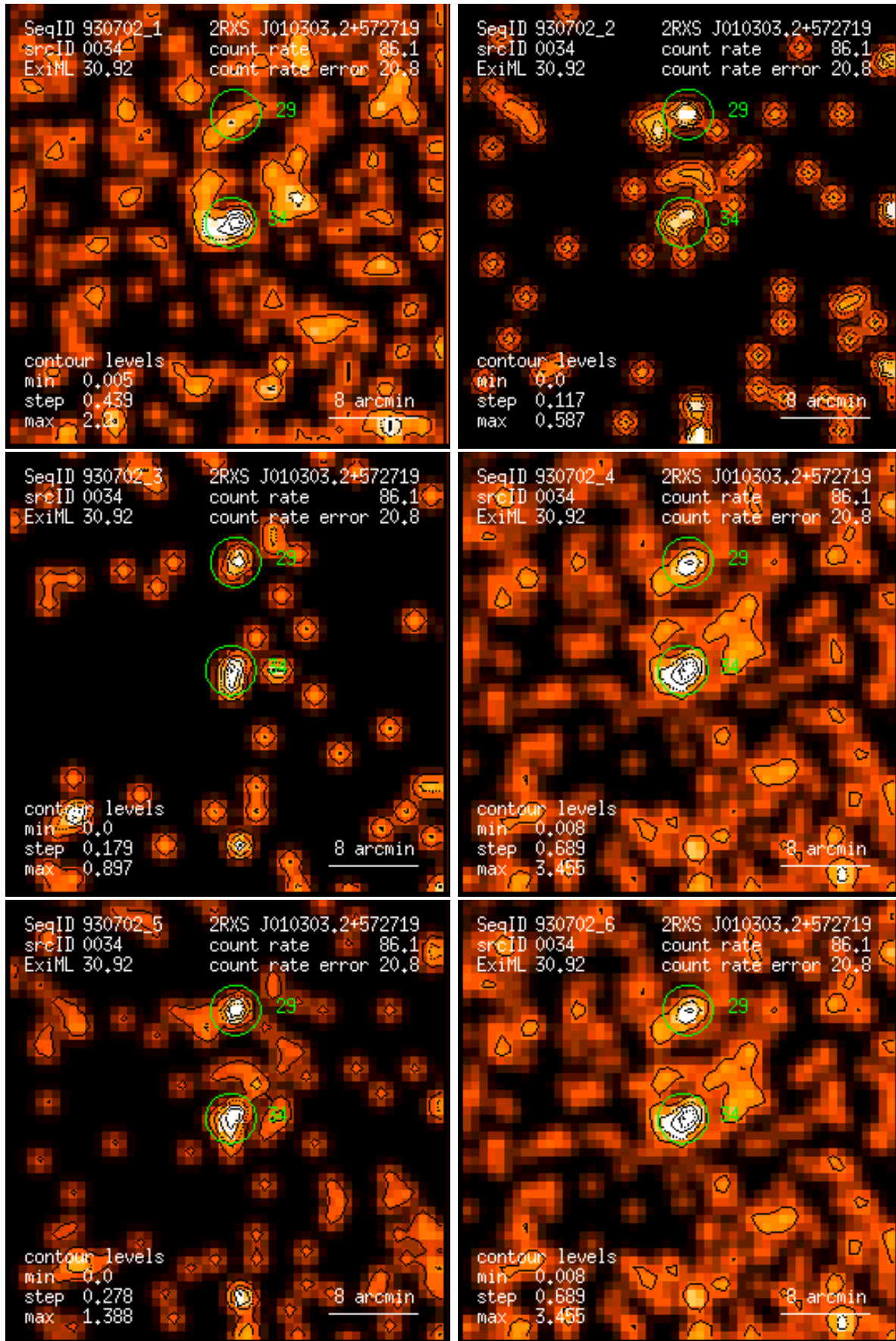
Figure 34: RASS 930702: detection 0034: band rate images, Gaussian filter: (1) PSPC channels 11 – 41, (2) 52 – 90, (3) 91 – 201, (4) 11 – 235, (5) 52 – 201, (6) 11 – 201. Broad band rates in counts/ks. Band rate contour levels in counts/ks/arcmin 2 .
