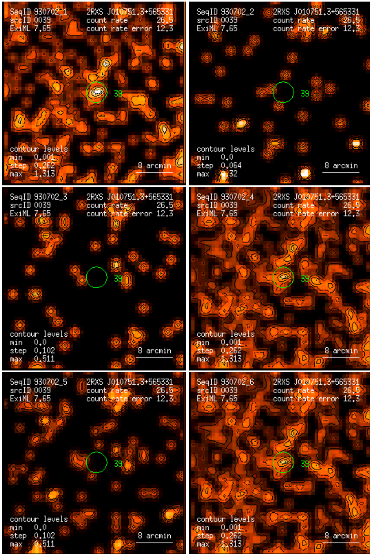
Figure 39: RASS 930702: detection 0039: band rate images, Gaussian filter: (1) PSPC channels 11 – 41, (2) 52 – 90, (3) 91 – 201, (4) 11 – 235, (5) 52 – 201, (6) 11 – 201. Broad band rates in counts/ks. Band rate contour levels in counts/ks/arcmin 2 .
