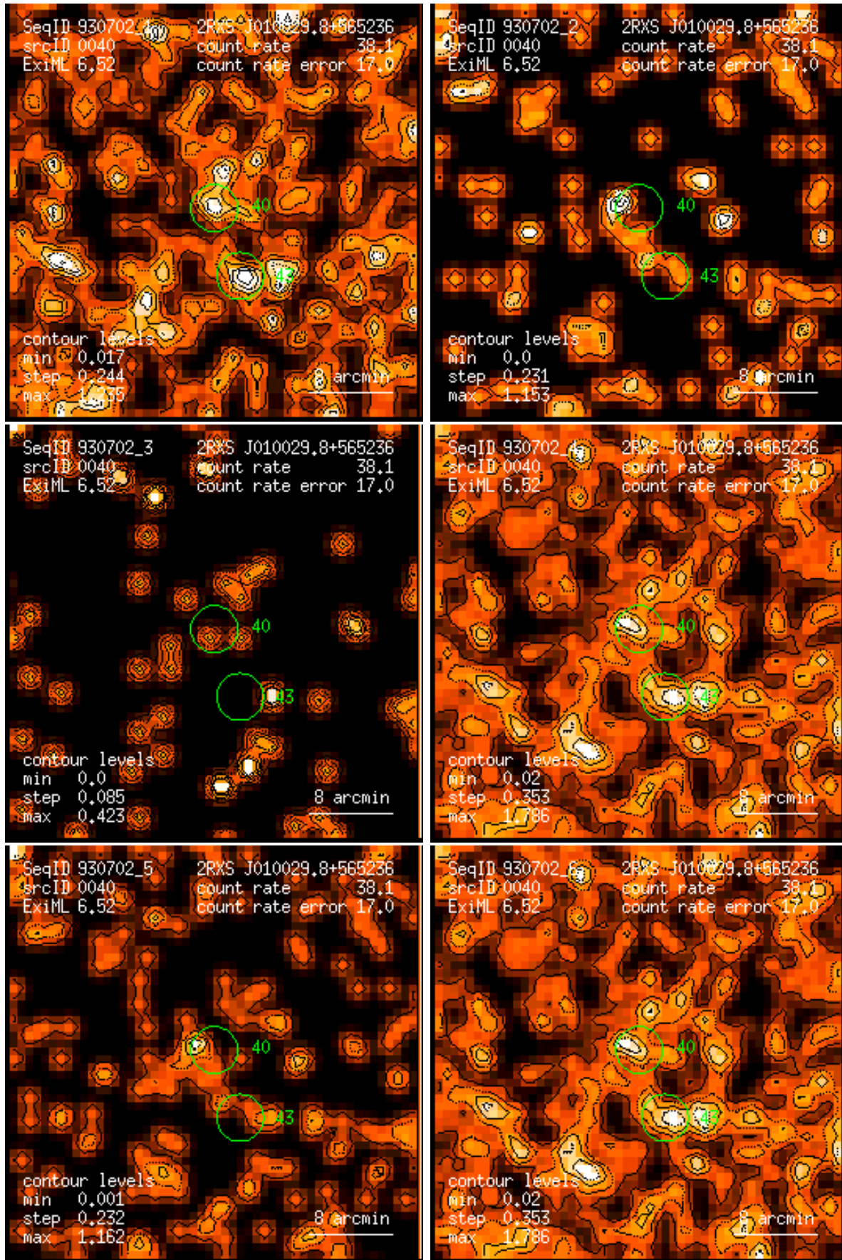
Figure 40: RASS 930702: detection 0040: band rate images, Gaussian filter: (1) PSPC channels 11 – 41, (2) 52 – 90, (3) 91 – 201, (4) 11 – 235, (5) 52 – 201, (6) 11 – 201. Broad band rates in counts/ks. Band rate contour levels in counts/ks/arcmin 2 .
