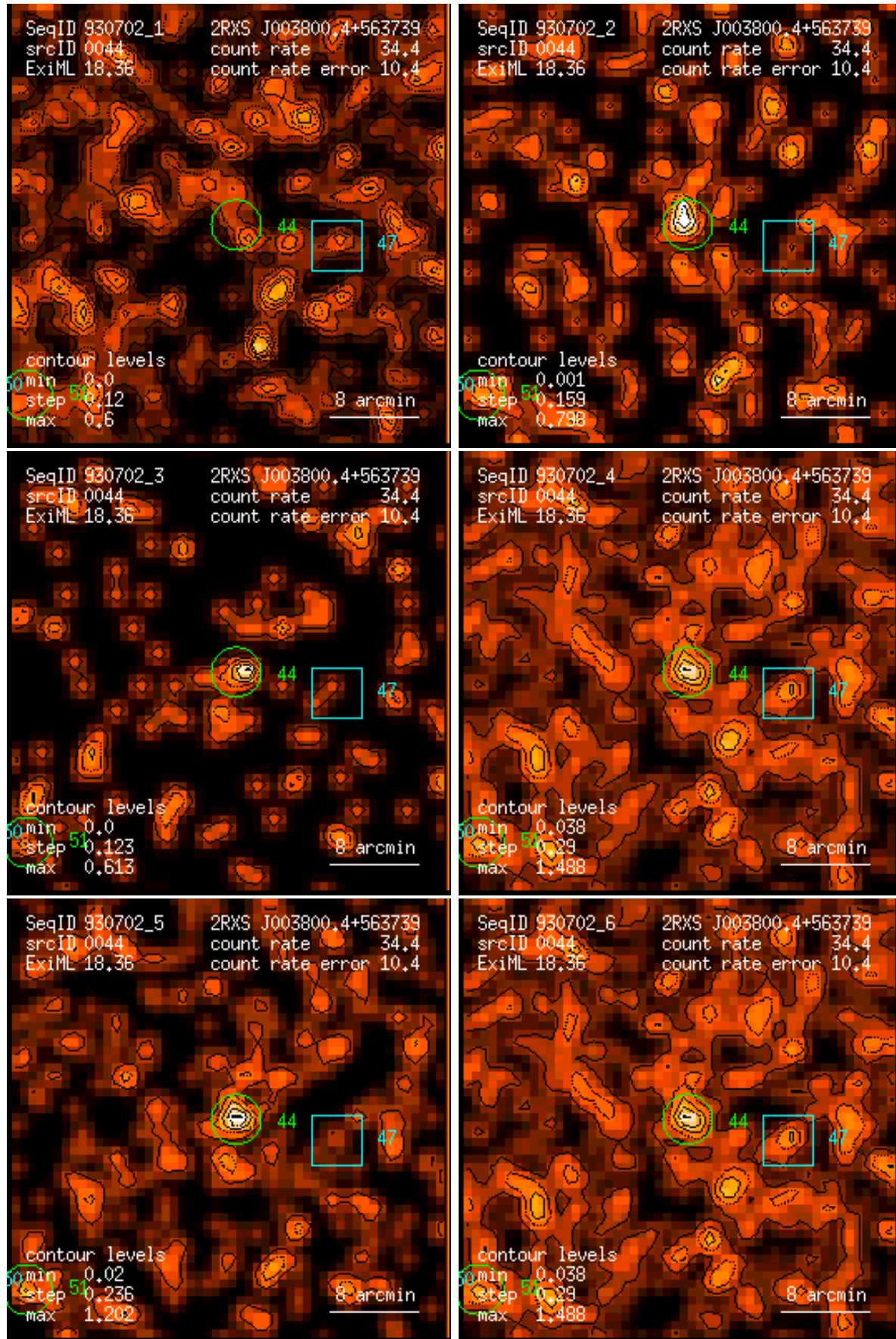
Figure 44: RASS 930702: detection 0044: band rate images, Gaussian filter: (1) PSPC channels 11 – 41, (2) 52 – 90, (3) 91 – 201, (4) 11 – 235, (5) 52 – 201, (6) 11 – 201. Broad band rates in counts/ks. Band rate contour levels in counts/ks/arcmin 2 .
