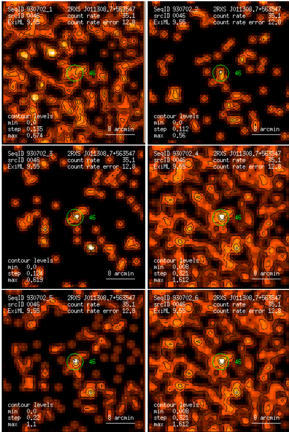
Figure 46: RASS 930702: detection 0046: band rate images, Gaussian filter: (1) PSPC channels 11 – 41, (2) 52 – 90, (3) 91 – 201, (4) 11 – 235, (5) 52 – 201, (6) 11 – 201. Broad band rates in counts/ks. Band rate contour levels in counts/ks/arcmin 2 .
