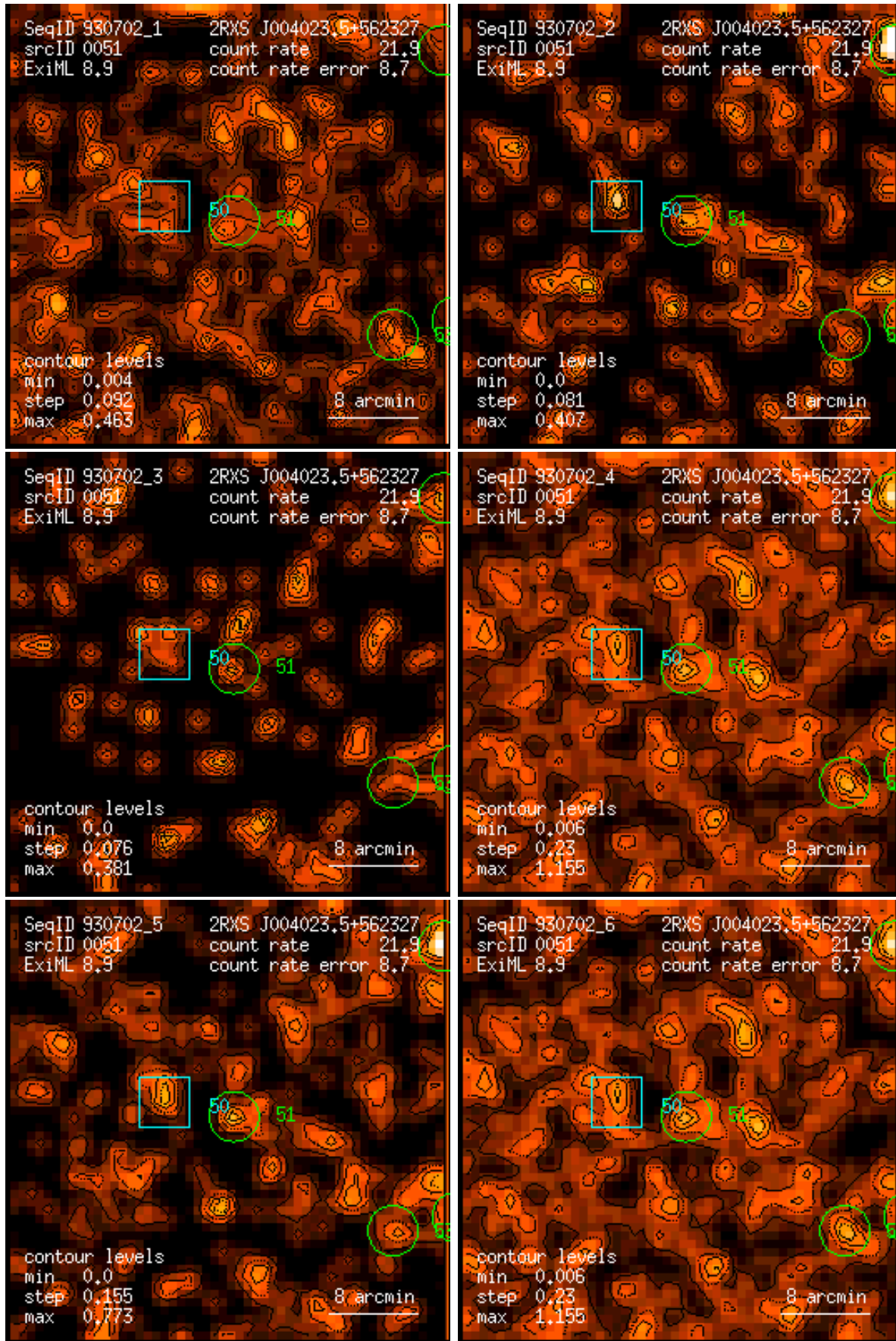
Figure 51: RASS 930702: detection 0051: band rate images, Gaussian filter: (1) PSPC channels 11 – 41, (2) 52 – 90, (3) 91 – 201, (4) 11 – 235, (5) 52 – 201, (6) 11 – 201. Broad band rates in counts/ks. Band rate contour levels in counts/ks/arcmin 2 .
