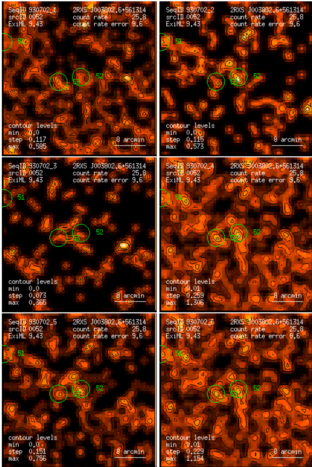
Figure 52: RASS 930702: detection 0052: band rate images, Gaussian filter: (1) PSPC channels 11 – 41, (2) 52 – 90, (3) 91 – 201, (4) 11 – 235, (5) 52 – 201, (6) 11 – 201. Broad band rates in counts/ks. Band rate contour levels in counts/ks/arcmin 2 .
