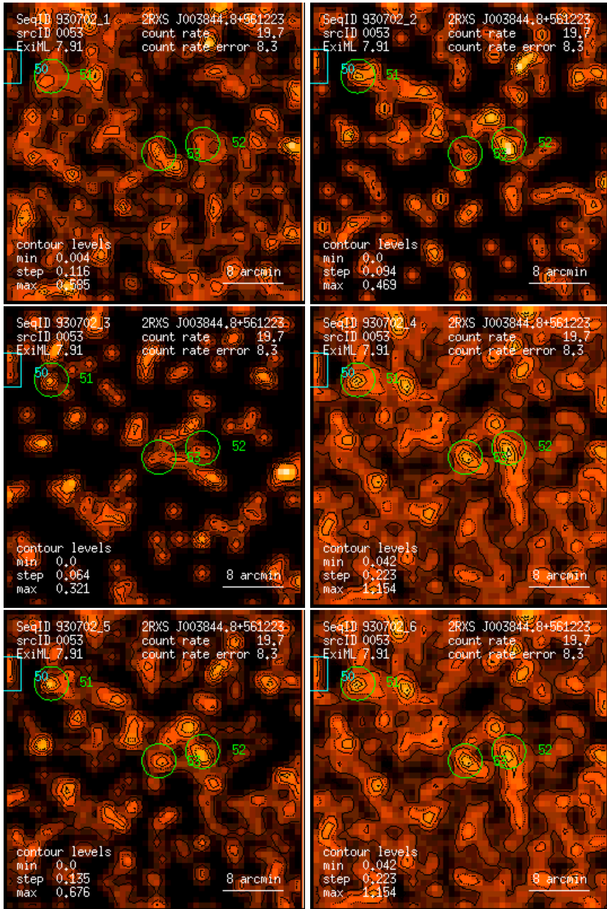
Figure 53: RASS 930702: detection 0053: band rate images, Gaussian filter: (1) PSPC channels 11 – 41, (2) 52 – 90, (3) 91 – 201, (4) 11 – 235, (5) 52 – 201, (6) 11 – 201. Broad band rates in counts/ks. Band rate contour levels in counts/ks/arcmin 2 .
