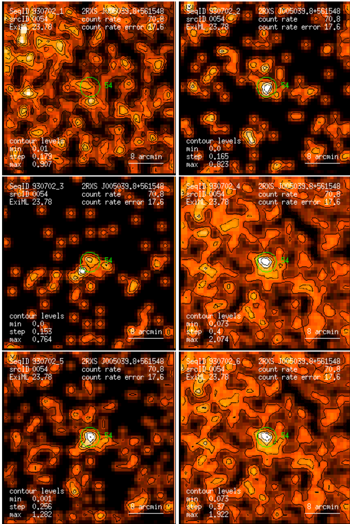
Figure 54: RASS 930702: detection 0054: band rate images, Gaussian filter: (1) PSPC channels 11 – 41, (2) 52 – 90, (3) 91 – 201, (4) 11 – 235, (5) 52 – 201, (6) 11 – 201. Broad band rates in counts/ks. Band rate contour levels in counts/ks/arcmin 2 .
