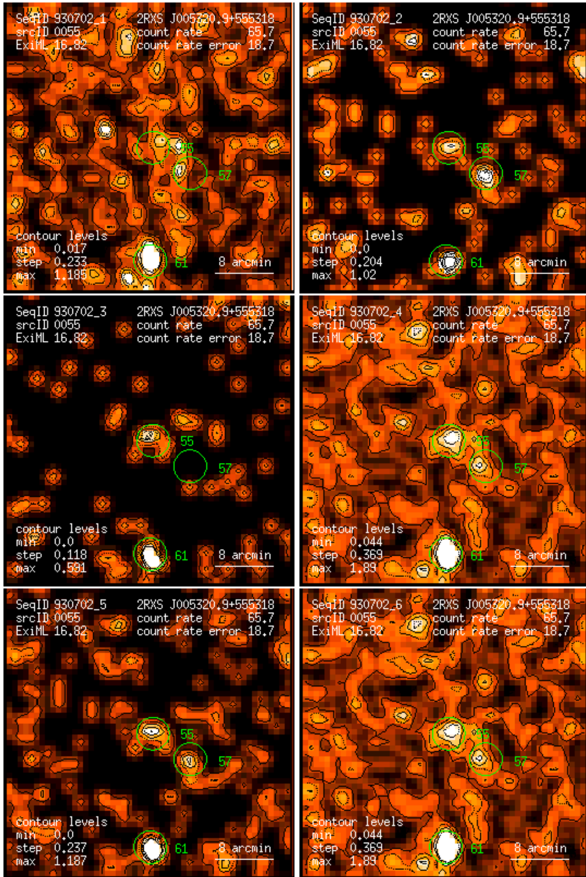
Figure 55: RASS 930702: detection 0055: band rate images, Gaussian filter: (1) PSPC channels 11 – 41, (2) 52 – 90, (3) 91 – 201, (4) 11 – 235, (5) 52 – 201, (6) 11 – 201. Broad band rates in counts/ks. Band rate contour levels in counts/ks/arcmin 2 .
