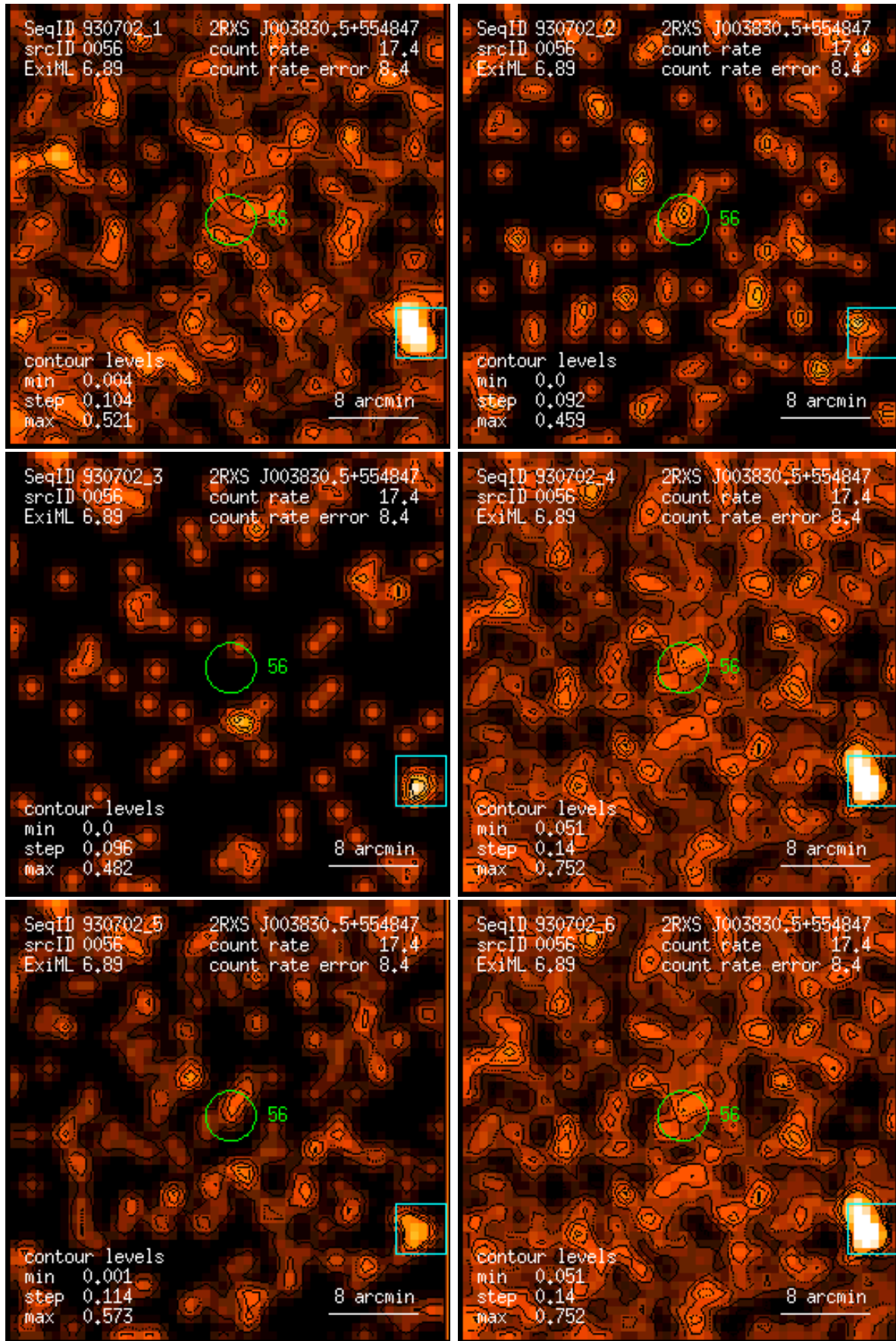
Figure 56: RASS 930702: detection 0056: band rate images, Gaussian filter: (1) PSPC channels 11 – 41, (2) 52 – 90, (3) 91 – 201, (4) 11 – 235, (5) 52 – 201, (6) 11 – 201. Broad band rates in counts/ks. Band rate contour levels in counts/ks/arcmin 2 .
