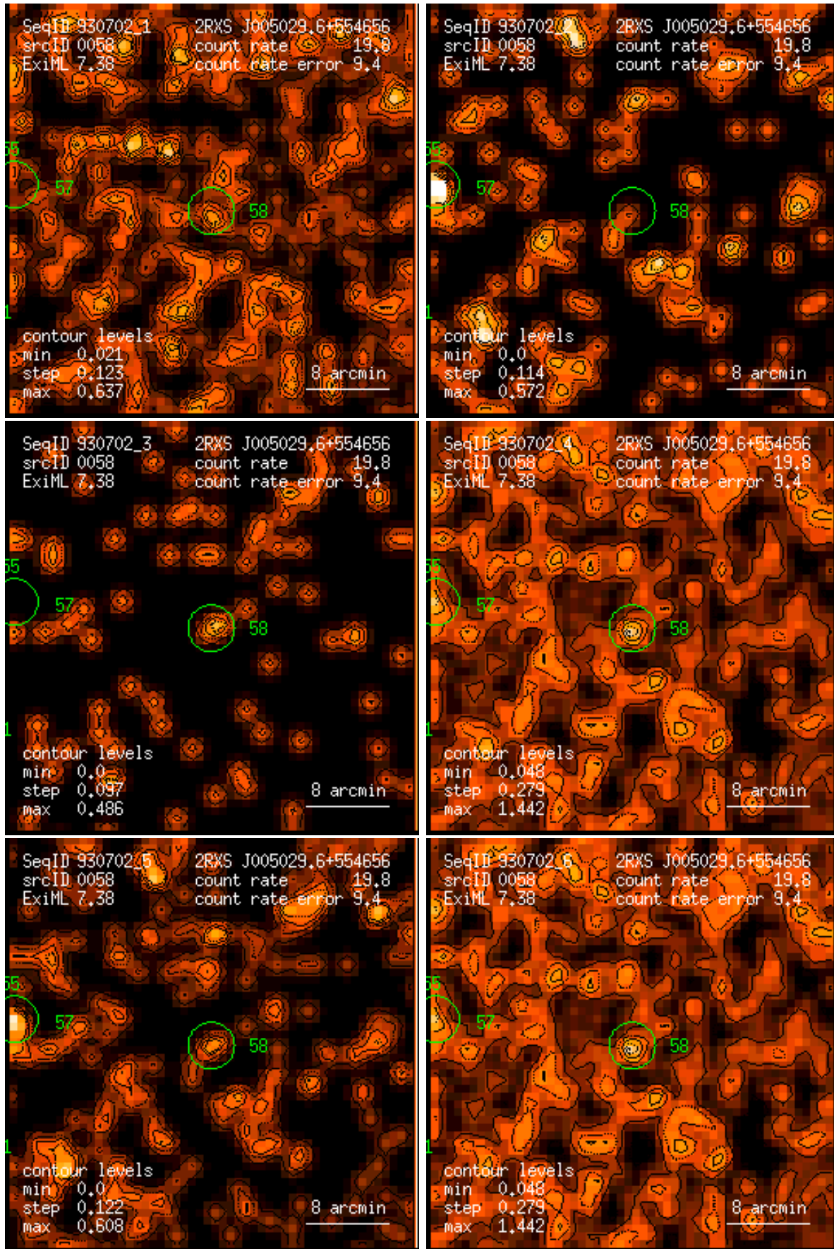
Figure 58: RASS 930702: detection 0058: band rate images, Gaussian filter: (1) PSPC channels 11 – 41, (2) 52 – 90, (3) 91 – 201, (4) 11 – 235, (5) 52 – 201, (6) 11 – 201. Broad band rates in counts/ks. Band rate contour levels in counts/ks/arcmin 2 .
