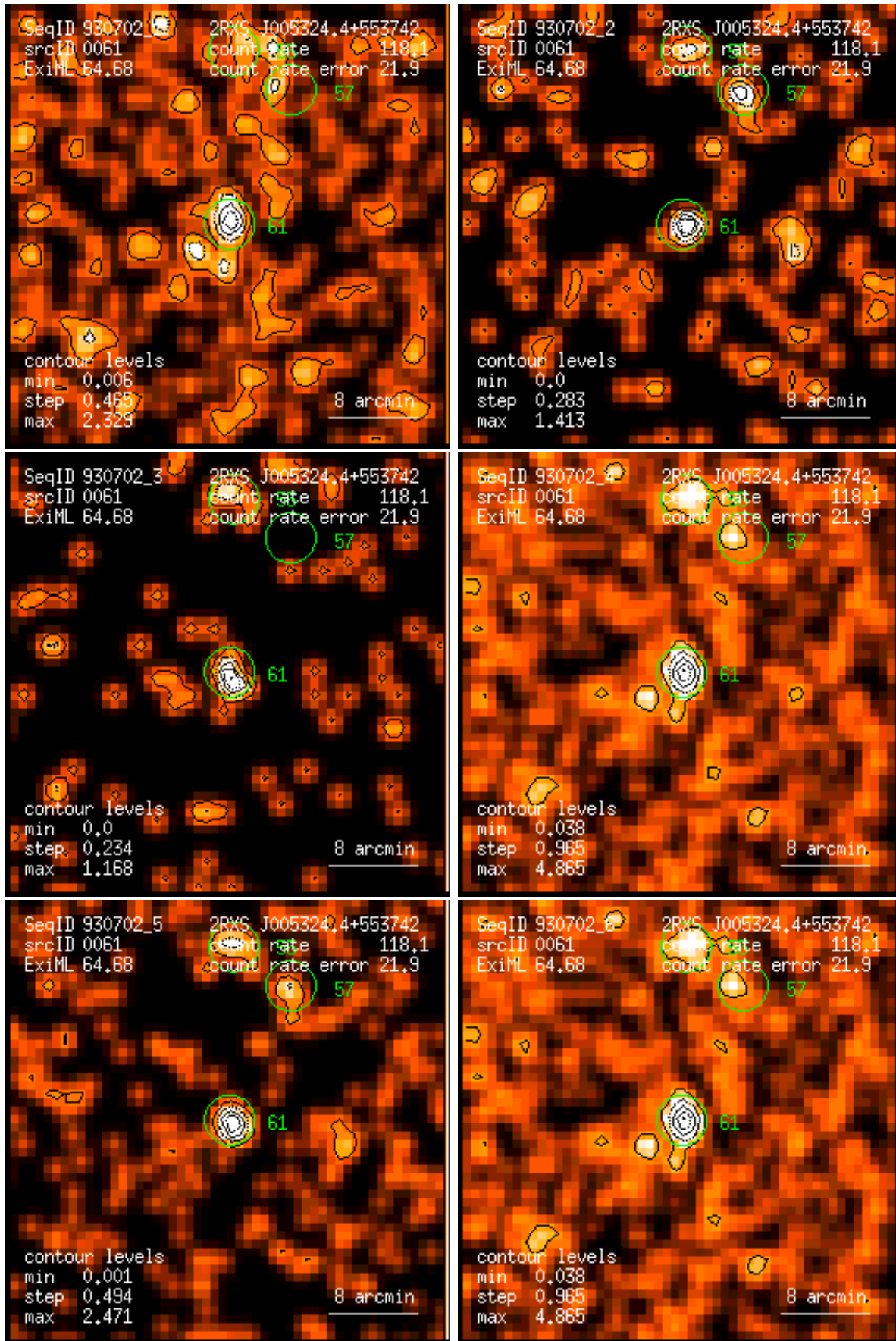
Figure 61: RASS 930702: detection 0061: band rate images, Gaussian filter: (1) PSPC channels 11 – 41, (2) 52 – 90, (3) 91 – 201, (4) 11 – 235, (5) 52 – 201, (6) 11 – 201. Broad band rates in counts/ks. Band rate contour levels in counts/ks/arcmin 2 .
