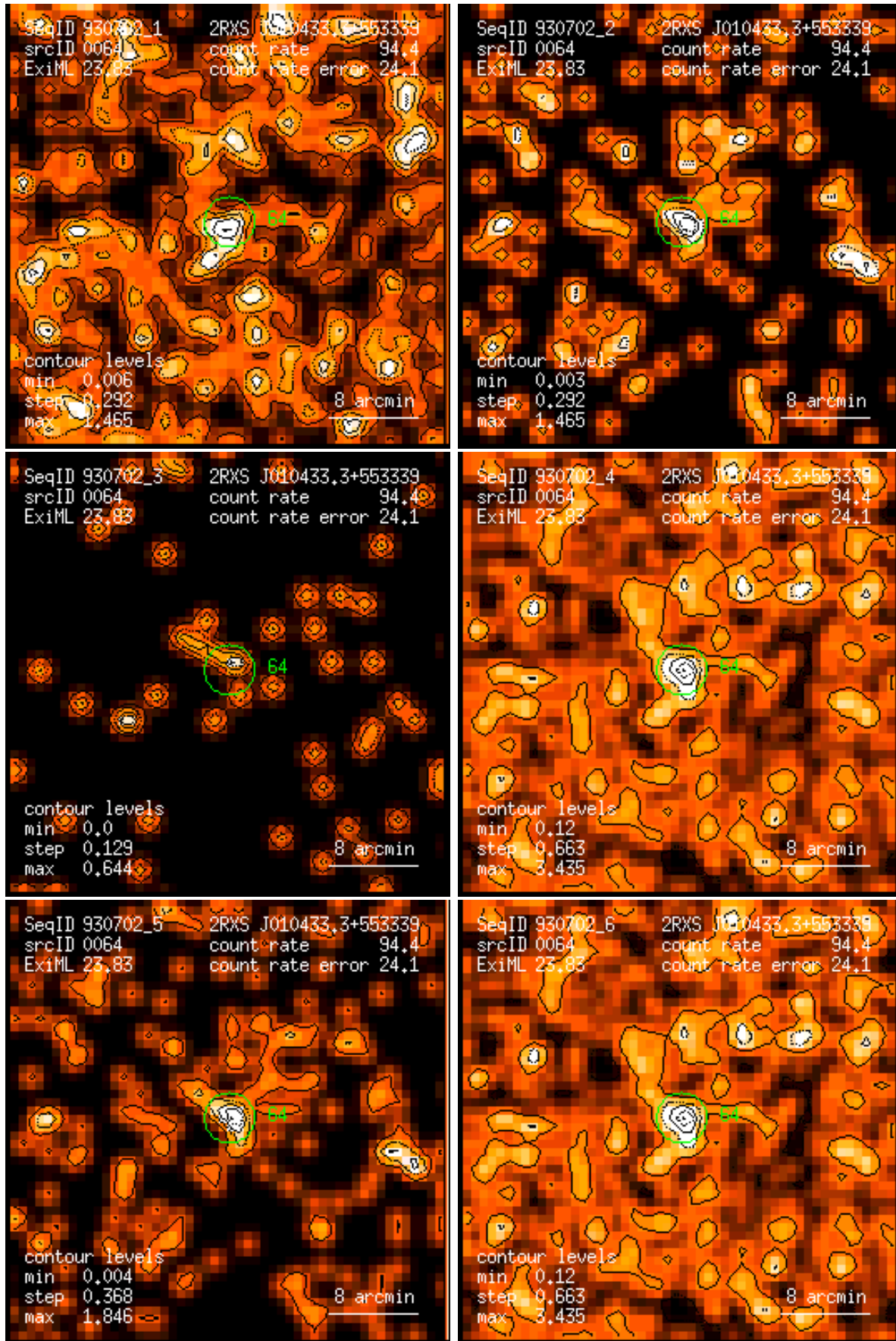
Figure 64: RASS 930702: detection 0064: band rate images, Gaussian filter: (1) PSPC channels 11 – 41, (2) 52 – 90, (3) 91 – 201, (4) 11 – 235, (5) 52 – 201, (6) 11 – 201. Broad band rates in counts/ks. Band rate contour levels in counts/ks/arcmin 2 .
