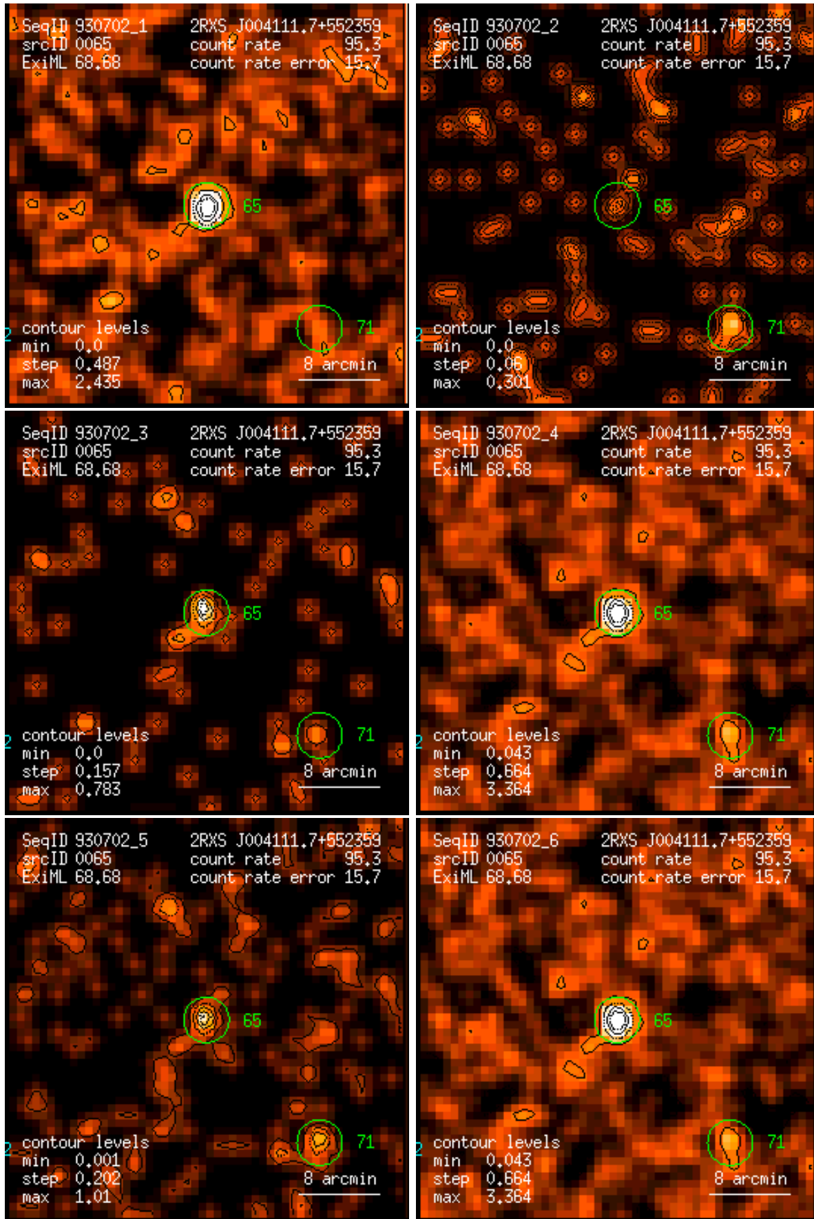
Figure 65: RASS 930702: detection 0065: band rate images, Gaussian filter: (1) PSPC channels 11 – 41, (2) 52 – 90, (3) 91 – 201, (4) 11 – 235, (5) 52 – 201, (6) 11 – 201. Broad band rates in counts/ks. Band rate contour levels in counts/ks/arcmin 2 .
