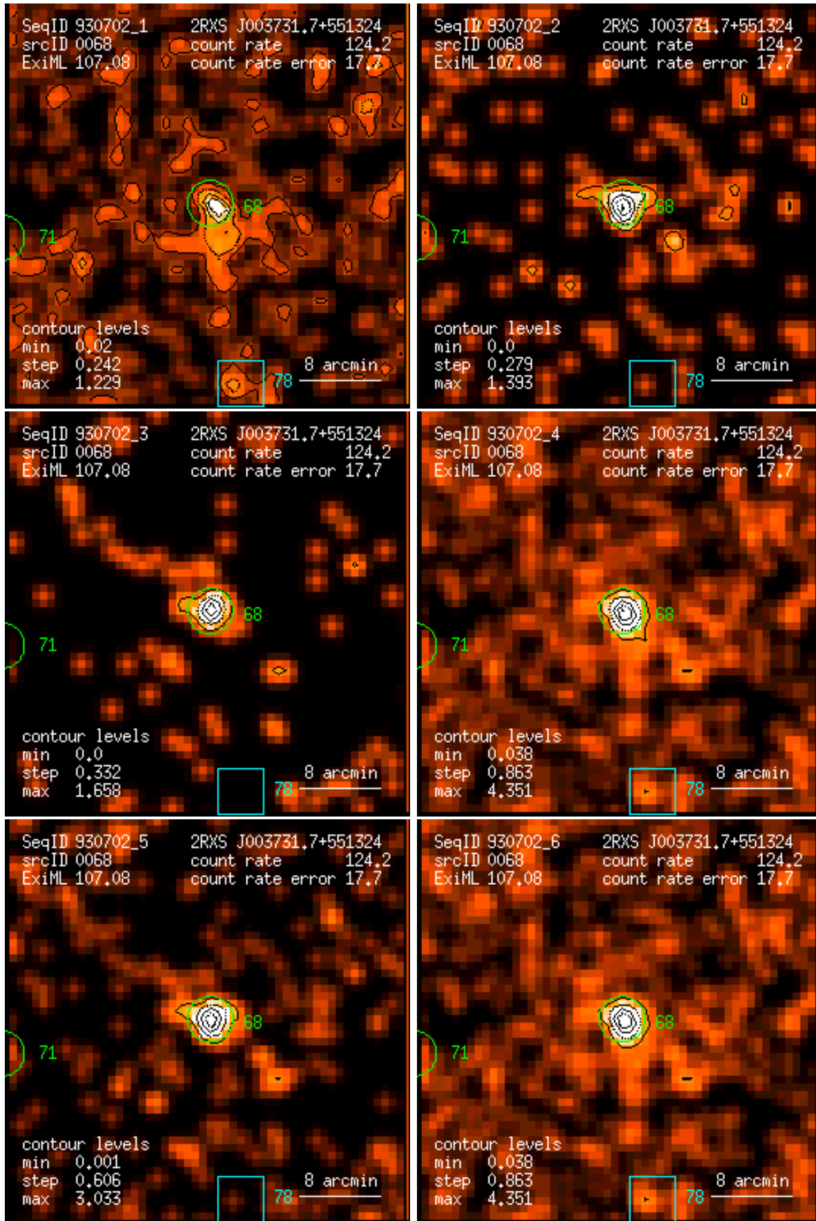
Figure 68: RASS 930702: detection 0068: band rate images, Gaussian filter: (1) PSPC channels 11 – 41, (2) 52 – 90, (3) 91 – 201, (4) 11 – 235, (5) 52 – 201, (6) 11 – 201. Broad band rates in counts/ks. Band rate contour levels in counts/ks/arcmin 2 .
