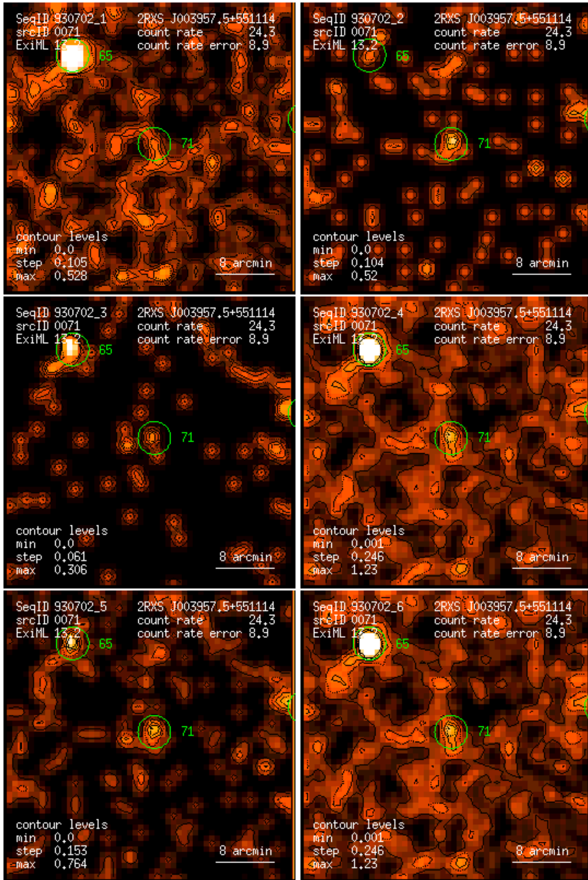
Figure 71: RASS 930702: detection 0071: band rate images, Gaussian filter: (1) PSPC channels 11 – 41, (2) 52 – 90, (3) 91 – 201, (4) 11 – 235, (5) 52 – 201, (6) 11 – 201. Broad band rates in counts/ks. Band rate contour levels in counts/ks/arcmin 2 .
