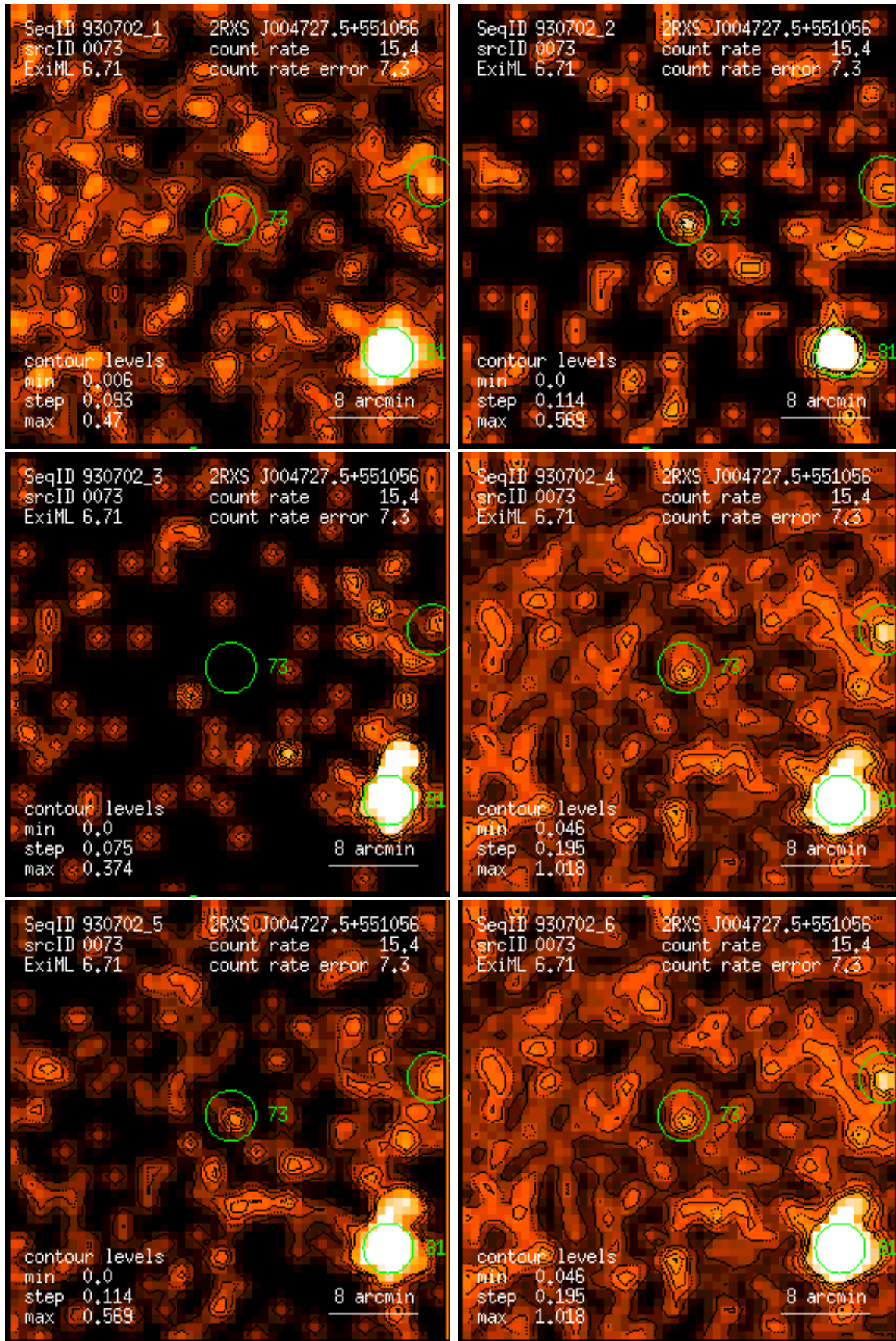
Figure 73: RASS 930702: detection 0073: band rate images, Gaussian filter: (1) PSPC channels 11 – 41, (2) 52 – 90, (3) 91 – 201, (4) 11 – 235, (5) 52 – 201, (6) 11 – 201. Broad band rates in counts/ks. Band rate contour levels in counts/ks/arcmin 2 .
