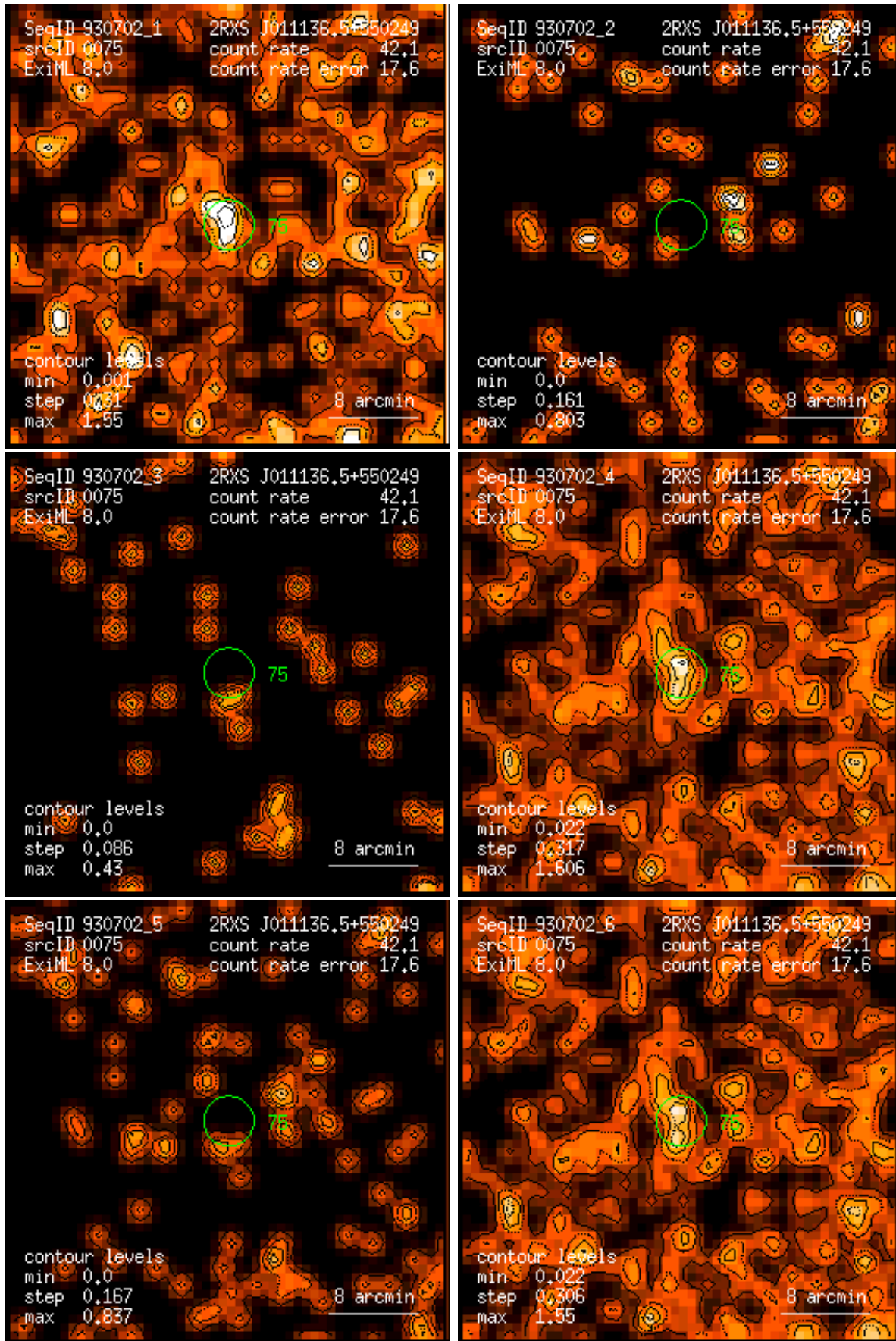
Figure 75: RASS 930702: detection 0075: band rate images, Gaussian filter: (1) PSPC channels 11 – 41, (2) 52 – 90, (3) 91 – 201, (4) 11 – 235, (5) 52 – 201, (6) 11 – 201. Broad band rates in counts/ks. Band rate contour levels in counts/ks/arcmin 2 .
