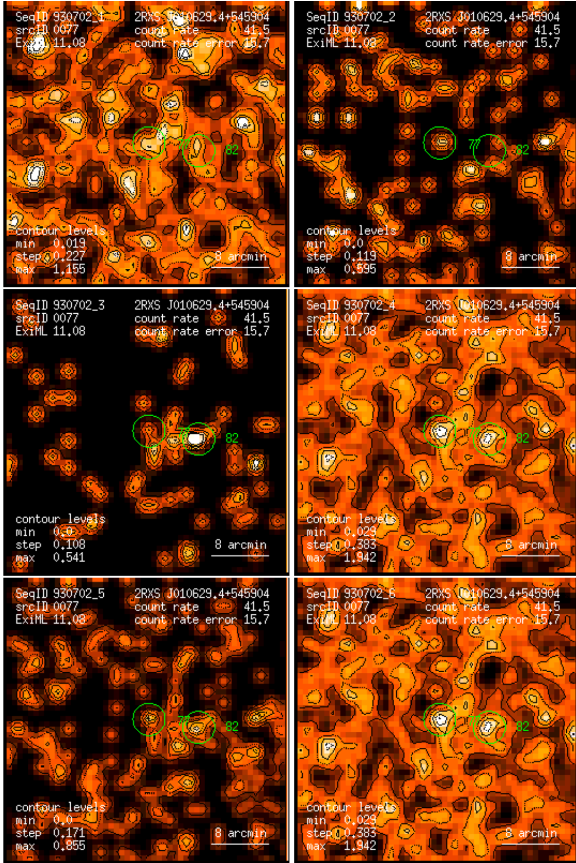
Figure 77: RASS 930702: detection 0077: band rate images, Gaussian filter: (1) PSPC channels 11 – 41, (2) 52 – 90, (3) 91 – 201, (4) 11 – 235, (5) 52 – 201, (6) 11 – 201. Broad band rates in counts/ks. Band rate contour levels in counts/ks/arcmin 2 .
