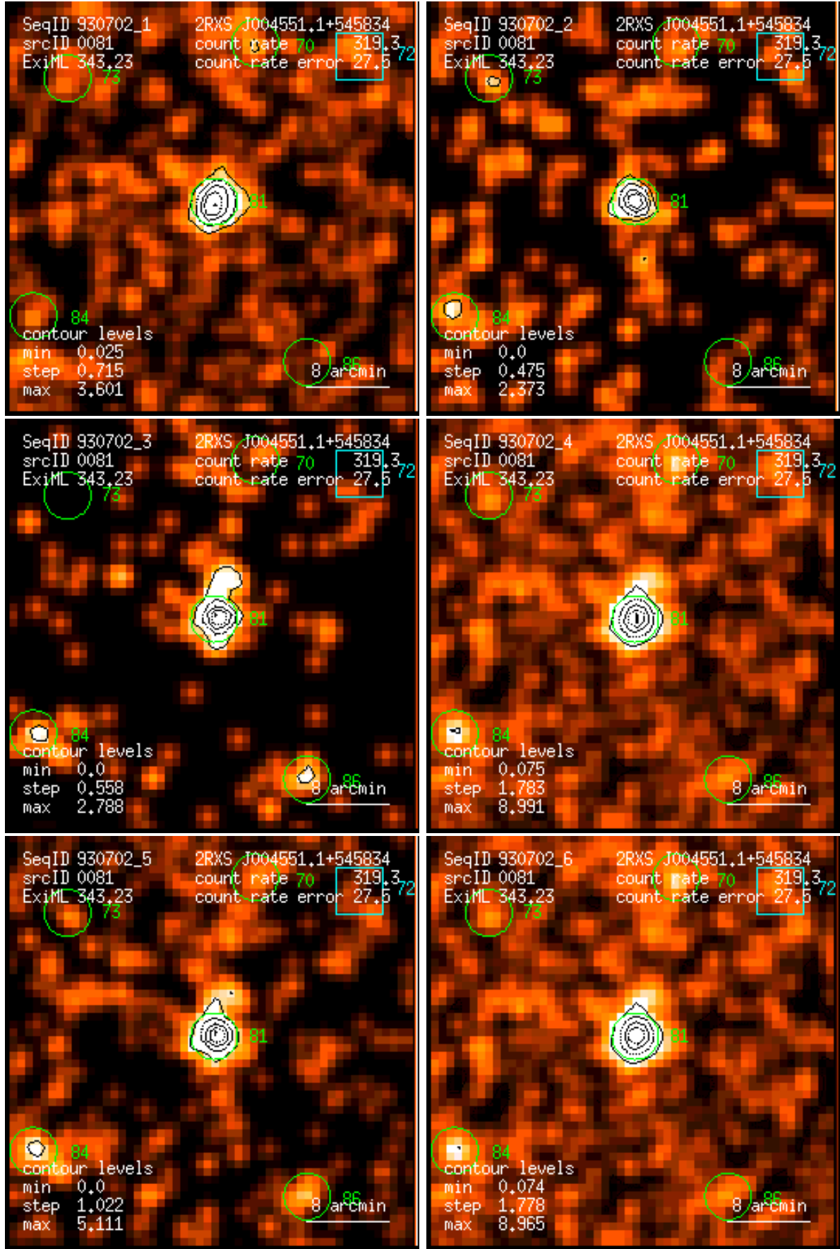
Figure 81: RASS 930702: detection 0081: band rate images, Gaussian filter: (1) PSPC channels 11 – 41, (2) 52 – 90, (3) 91 – 201, (4) 11 – 235, (5) 52 – 201, (6) 11 – 201. Broad band rates in counts/ks. Band rate contour levels in counts/ks/arcmin 2 .
