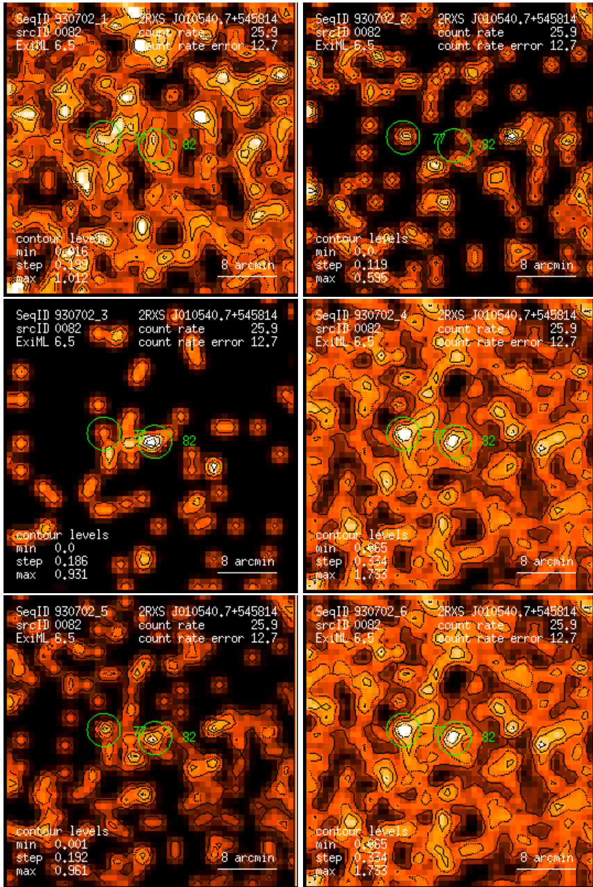
Figure 82: RASS 930702: detection 0082: band rate images, Gaussian filter: (1) PSPC channels 11 – 41, (2) 52 – 90, (3) 91 – 201, (4) 11 – 235, (5) 52 – 201, (6) 11 – 201. Broad band rates in counts/ks. Band rate contour levels in counts/ks/arcmin 2 .
