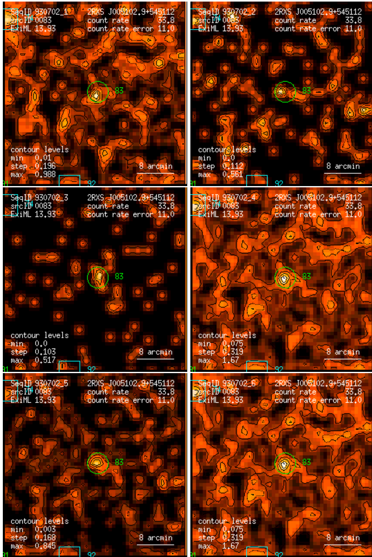
Figure 83: RASS 930702: detection 0083: band rate images, Gaussian filter: (1) PSPC channels 11 – 41, (2) 52 – 90, (3) 91 – 201, (4) 11 – 235, (5) 52 – 201, (6) 11 – 201. Broad band rates in counts/ks. Band rate contour levels in counts/ks/arcmin 2 .
