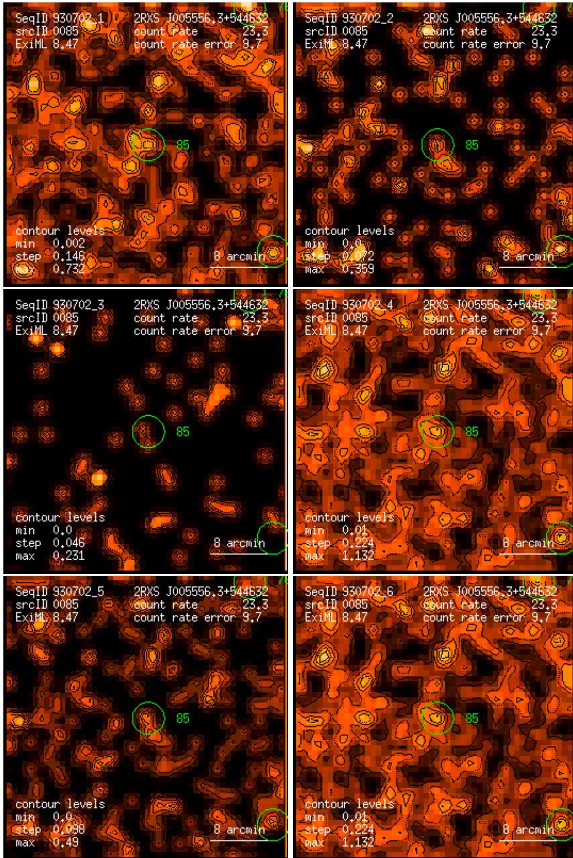
Figure 85: RASS 930702: detection 0085: band rate images, Gaussian filter: (1) PSPC channels 11 – 41, (2) 52 – 90, (3) 91 – 201, (4) 11 – 235, (5) 52 – 201, (6) 11 – 201. Broad band rates in counts/ks. Band rate contour levels in counts/ks/arcmin 2 .
