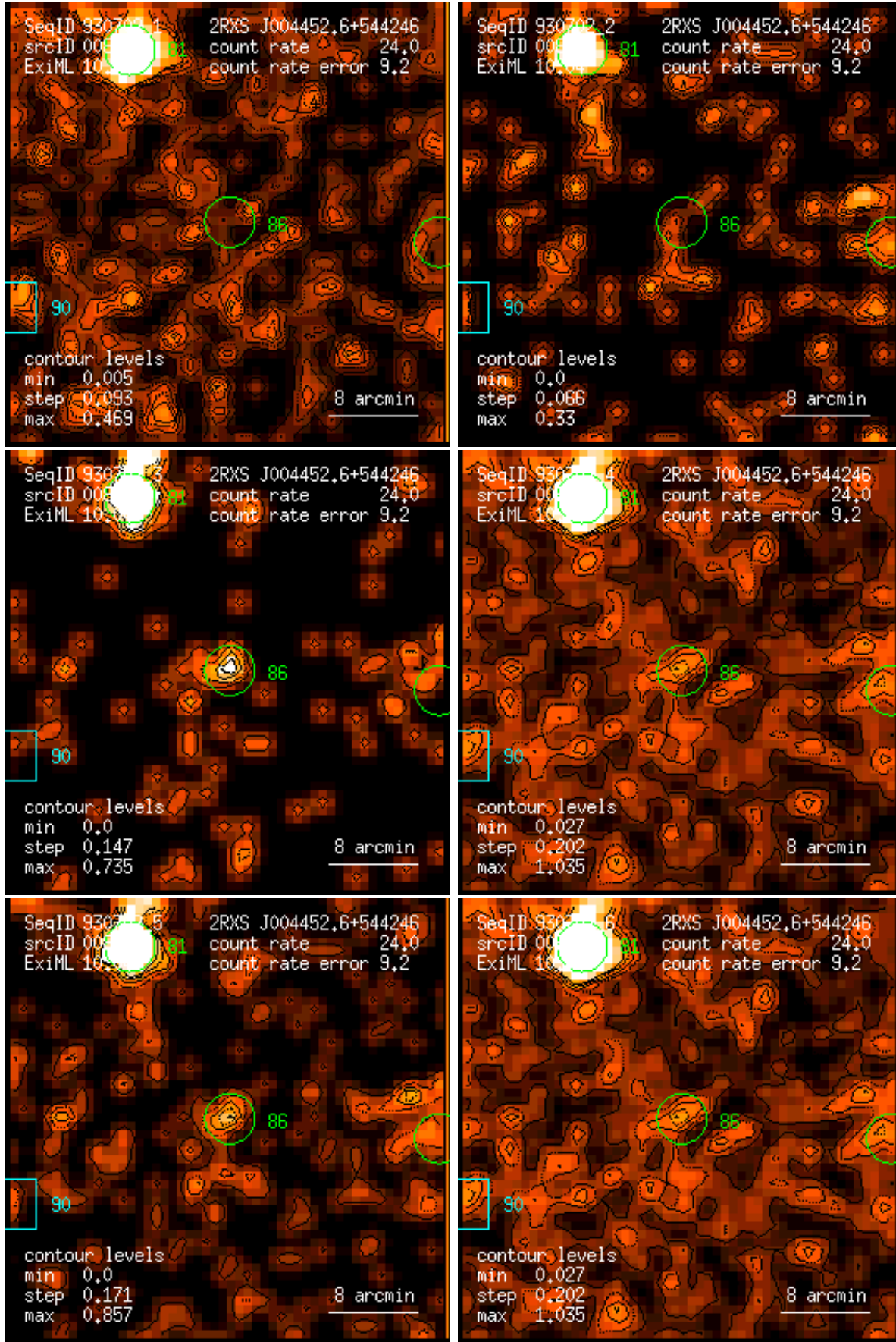
Figure 86: RASS 930702: detection 0086: band rate images, Gaussian filter: (1) PSPC channels 11 – 41, (2) 52 – 90, (3) 91 – 201, (4) 11 – 235, (5) 52 – 201, (6) 11 – 201. Broad band rates in counts/ks. Band rate contour levels in counts/ks/arcmin 2 .
