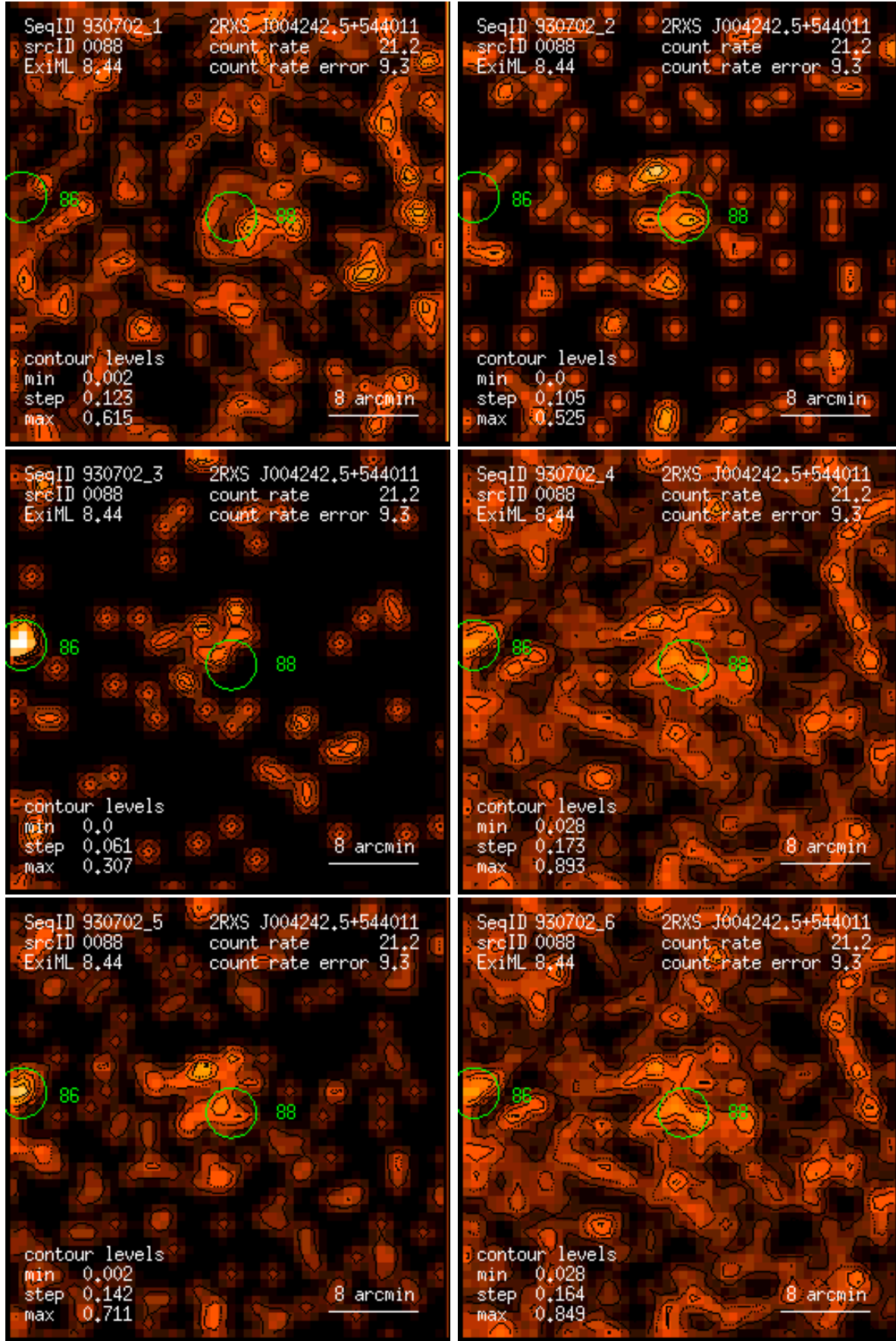
Figure 88: RASS 930702: detection 0088: band rate images, Gaussian filter: (1) PSPC channels 11 – 41, (2) 52 – 90, (3) 91 – 201, (4) 11 – 235, (5) 52 – 201, (6) 11 – 201. Broad band rates in counts/ks. Band rate contour levels in counts/ks/arcmin 2 .
