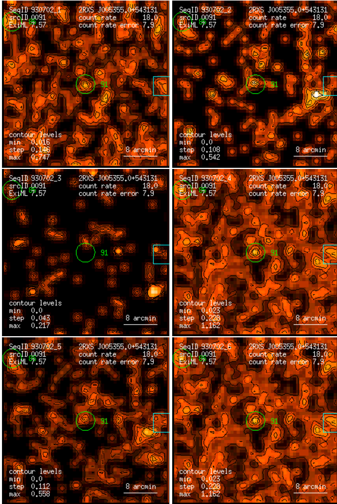
Figure 91: RASS 930702: detection 0091: band rate images, Gaussian filter: (1) PSPC channels 11 – 41, (2) 52 – 90, (3) 91 – 201, (4) 11 – 235, (5) 52 – 201, (6) 11 – 201. Broad band rates in counts/ks. Band rate contour levels in counts/ks/arcmin 2 .
