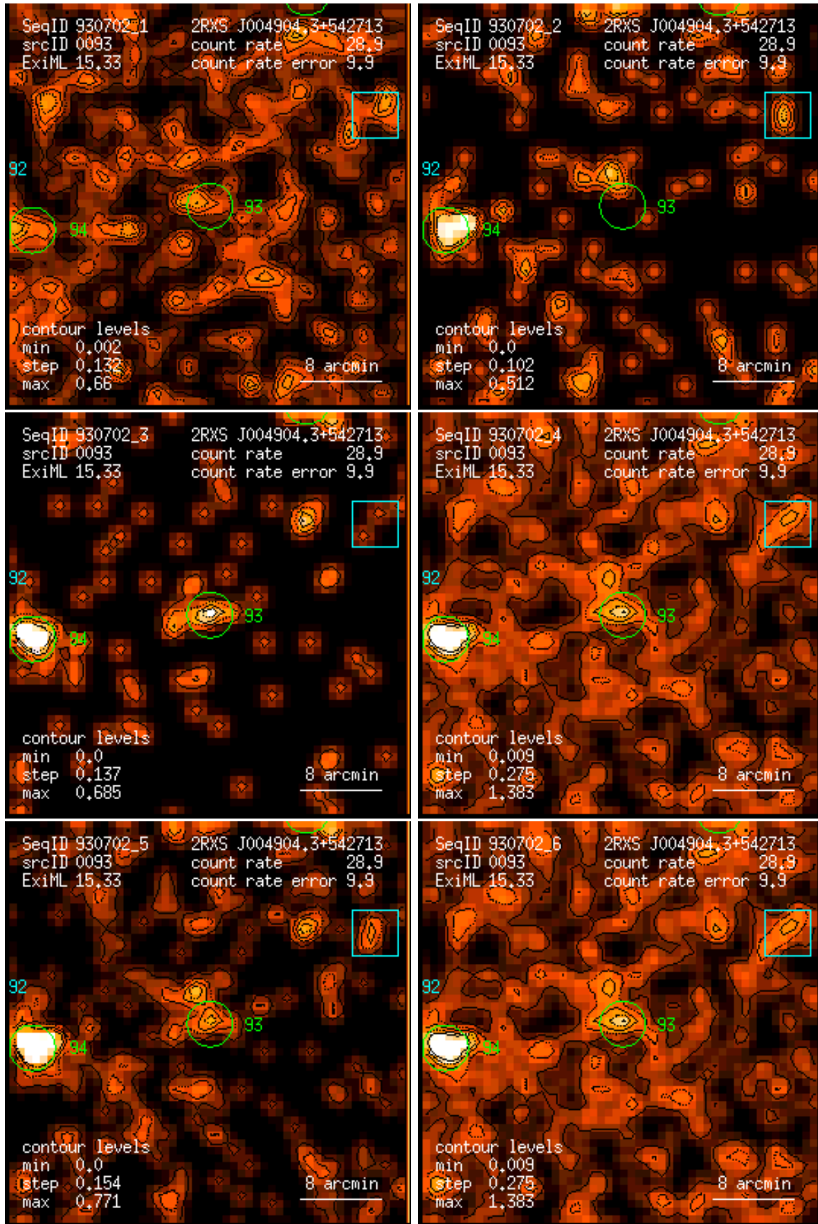
Figure 93: RASS 930702: detection 0093: band rate images, Gaussian filter: (1) PSPC channels 11 – 41, (2) 52 – 90, (3) 91 – 201, (4) 11 – 235, (5) 52 – 201, (6) 11 – 201. Broad band rates in counts/ks. Band rate contour levels in counts/ks/arcmin 2 .
