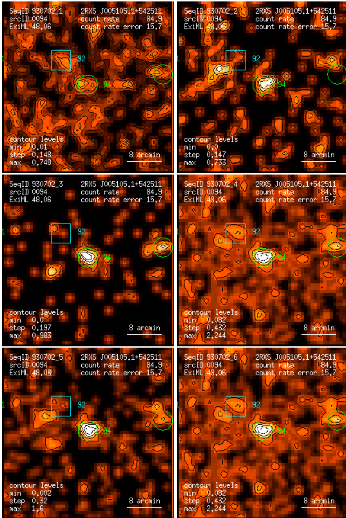
Figure 94: RASS 930702: detection 0094: band rate images, Gaussian filter: (1) PSPC channels 11 – 41, (2) 52 – 90, (3) 91 – 201, (4) 11 – 235, (5) 52 – 201, (6) 11 – 201. Broad band rates in counts/ks. Band rate contour levels in counts/ks/arcmin 2 .
