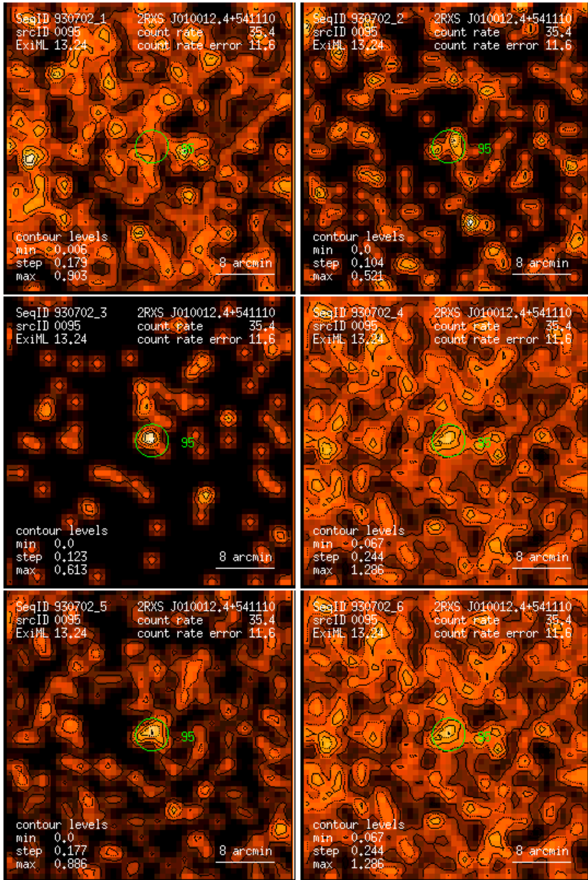
Figure 95: RASS 930702: detection 0095: band rate images, Gaussian filter: (1) PSPC channels 11 – 41, (2) 52 – 90, (3) 91 – 201, (4) 11 – 235, (5) 52 – 201, (6) 11 – 201. Broad band rates in counts/ks. Band rate contour levels in counts/ks/arcmin 2 .
