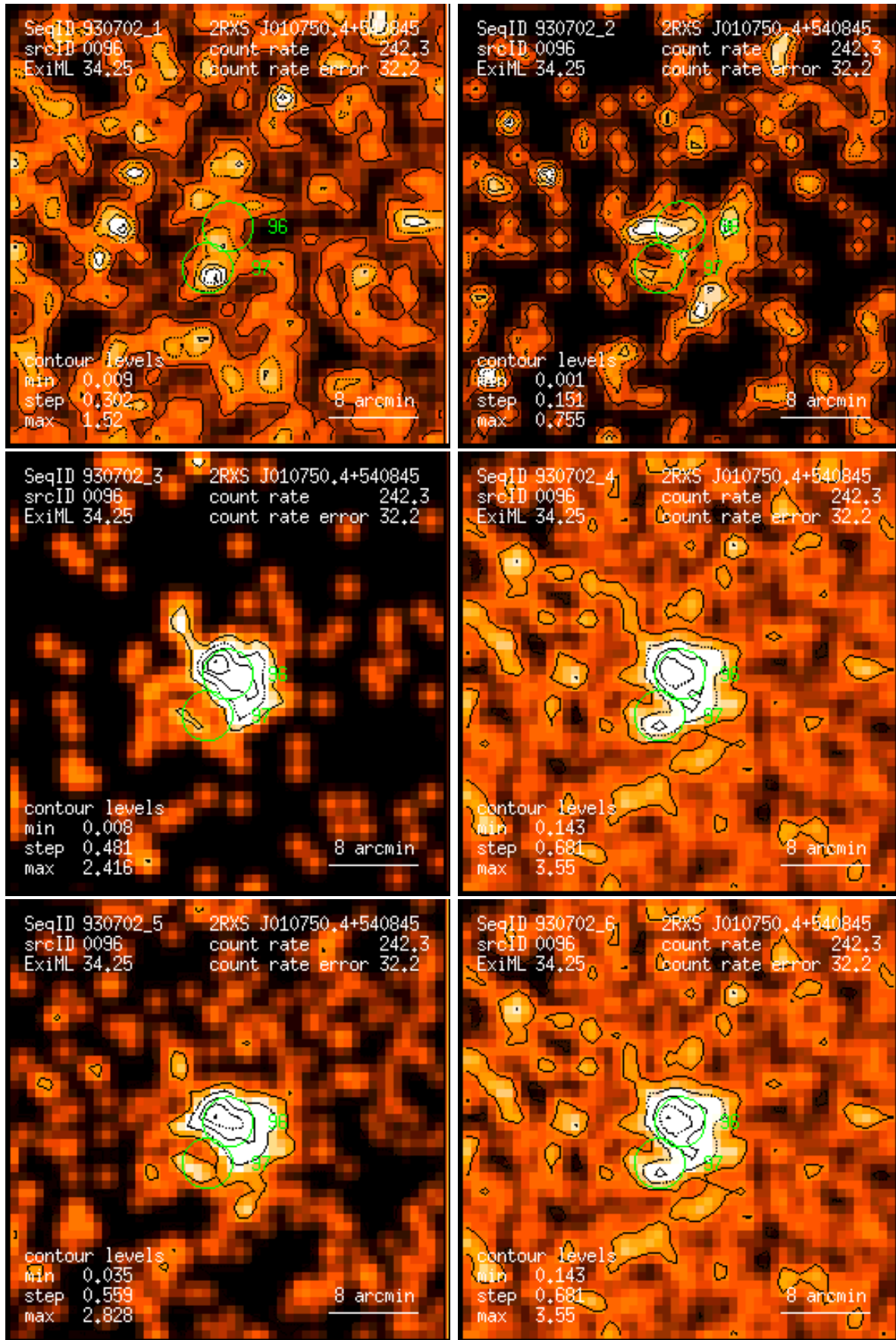
Figure 96: RASS 930702: detection 0096: band rate images, Gaussian filter: (1) PSPC channels 11 – 41, (2) 52 – 90, (3) 91 – 201, (4) 11 – 235, (5) 52 – 201, (6) 11 – 201. Broad band rates in counts/ks. Band rate contour levels in counts/ks/arcmin 2 .
