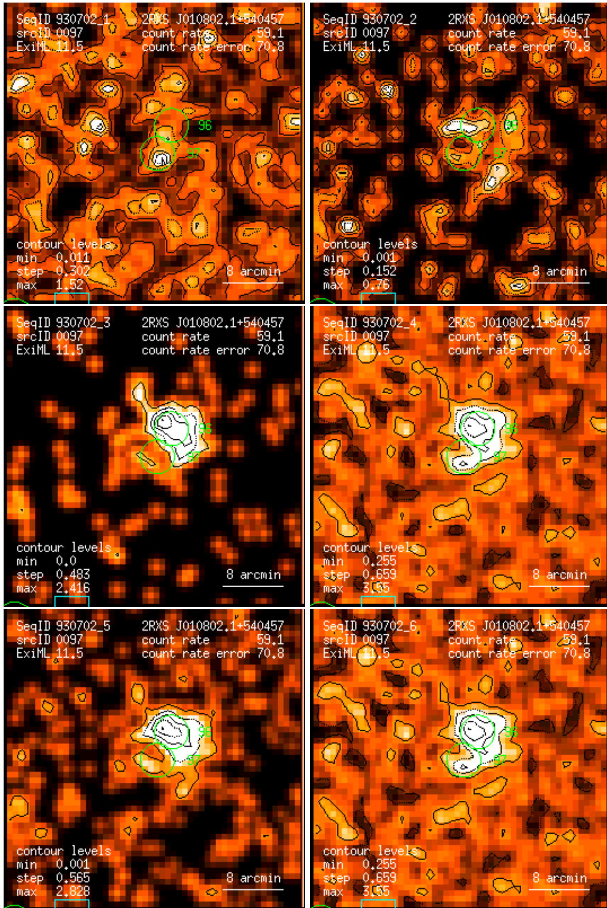
Figure 97: RASS 930702: detection 0097: band rate images, Gaussian filter: (1) PSPC channels 11 – 41, (2) 52 – 90, (3) 91 – 201, (4) 11 – 235, (5) 52 – 201, (6) 11 – 201. Broad band rates in counts/ks. Band rate contour levels in counts/ks/arcmin 2 .
