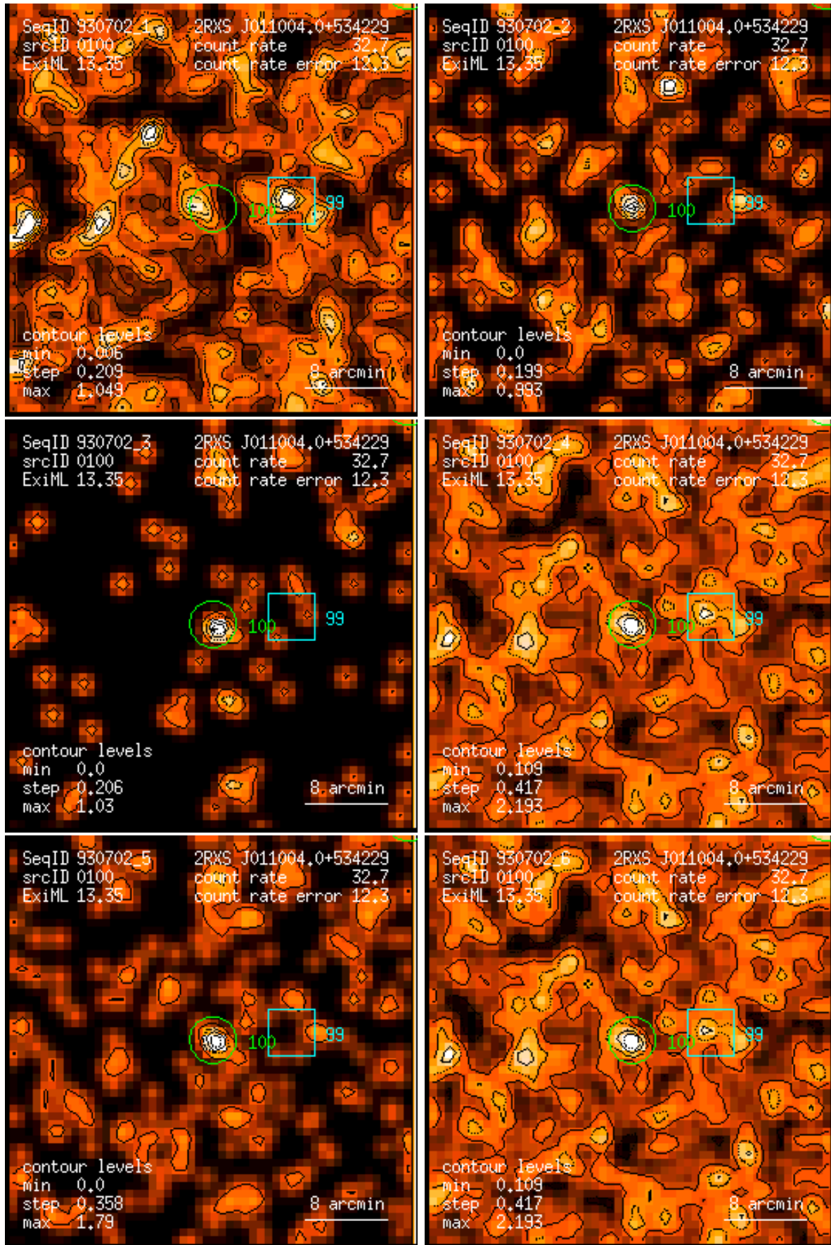
Figure 100: RASS 930702: detection 0100: band rate images, Gaussian filter: (1) PSPC channels 11 – 41, (2) 52 – 90, (3) 91 – 201, (4) 11 – 235, (5) 52 – 201, (6) 11 – 201. Broad band rates in counts/ks. Band rate contour levels in counts/ks/arcmin 2 .
