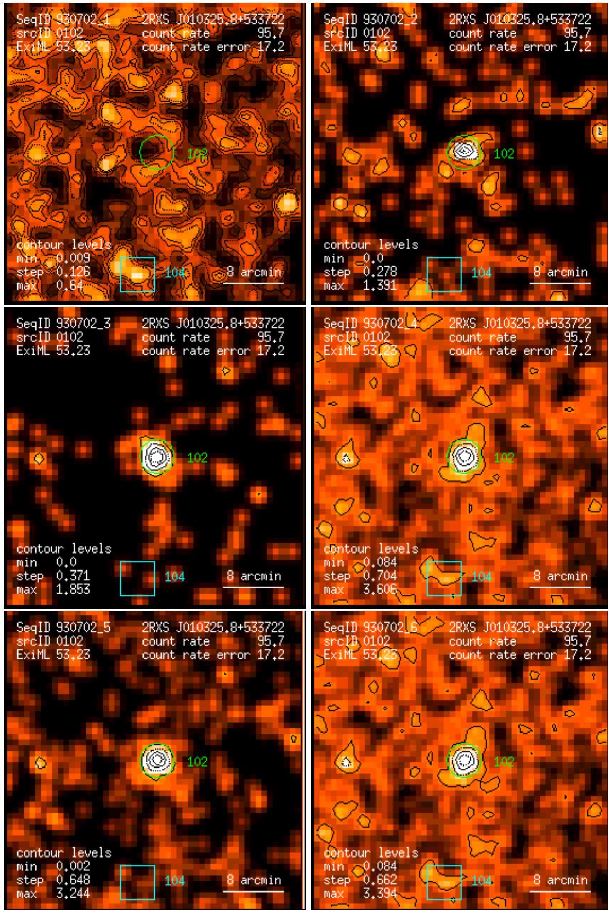
Figure 102: RASS 930702: detection 0102: band rate images, Gaussian filter: (1) PSPC channels 11 – 41, (2) 52 – 90, (3) 91 – 201, (4) 11 – 235, (5) 52 – 201, (6) 11 – 201. Broad band rates in counts/ks. Band rate contour levels in counts/ks/arcmin 2 .
