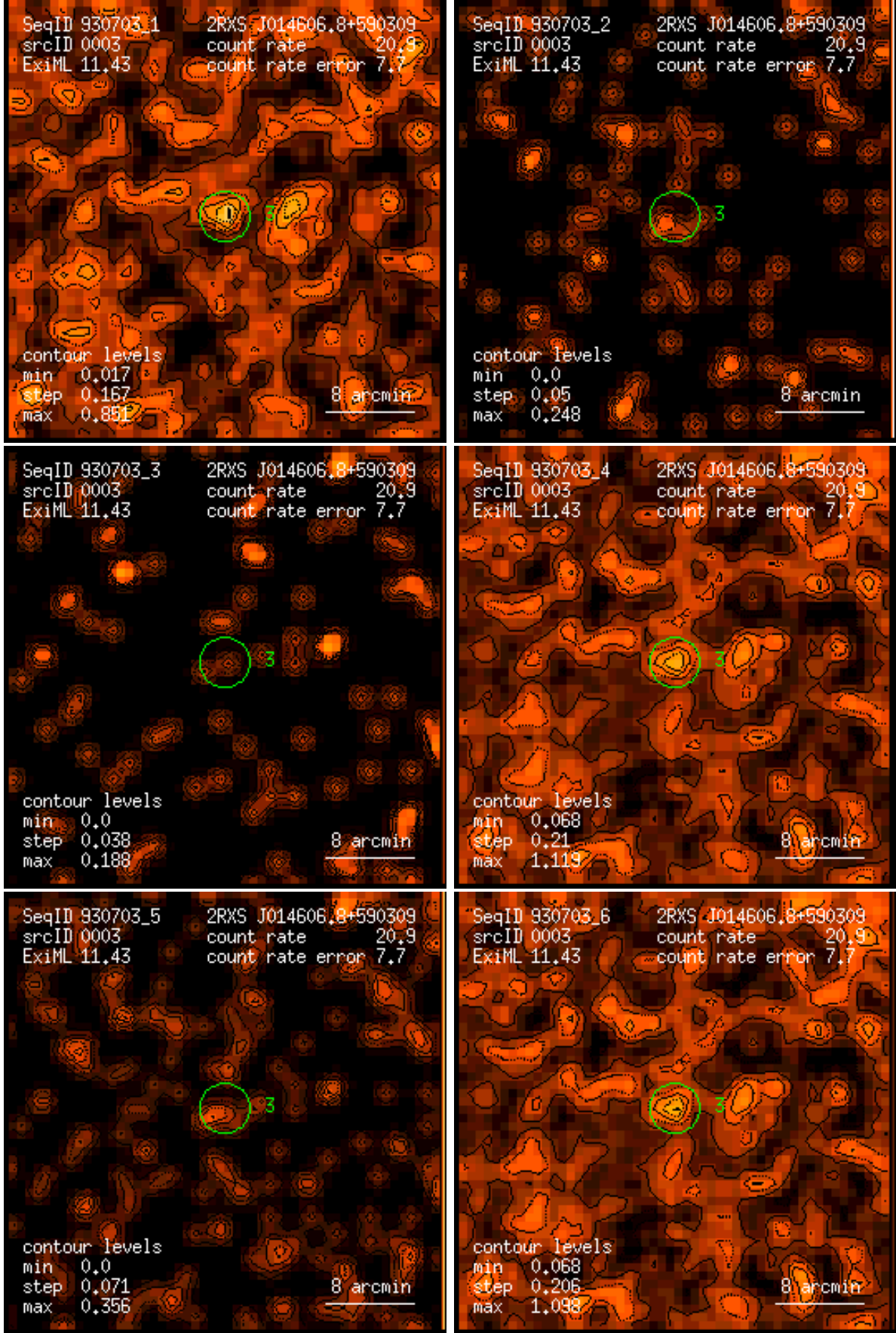
Figure 3: RASS 930703: detection 0003: band rate images, Gaussian filter: (1) PSPC channels 11 – 41, (2) 52 – 90, (3) 91 – 201, (4) 11 – 235, (5) 52 – 201, (6) 11 – 201. Broad band rates in counts/ks. Band rate contour levels in counts/ks/arcmin 2 .
