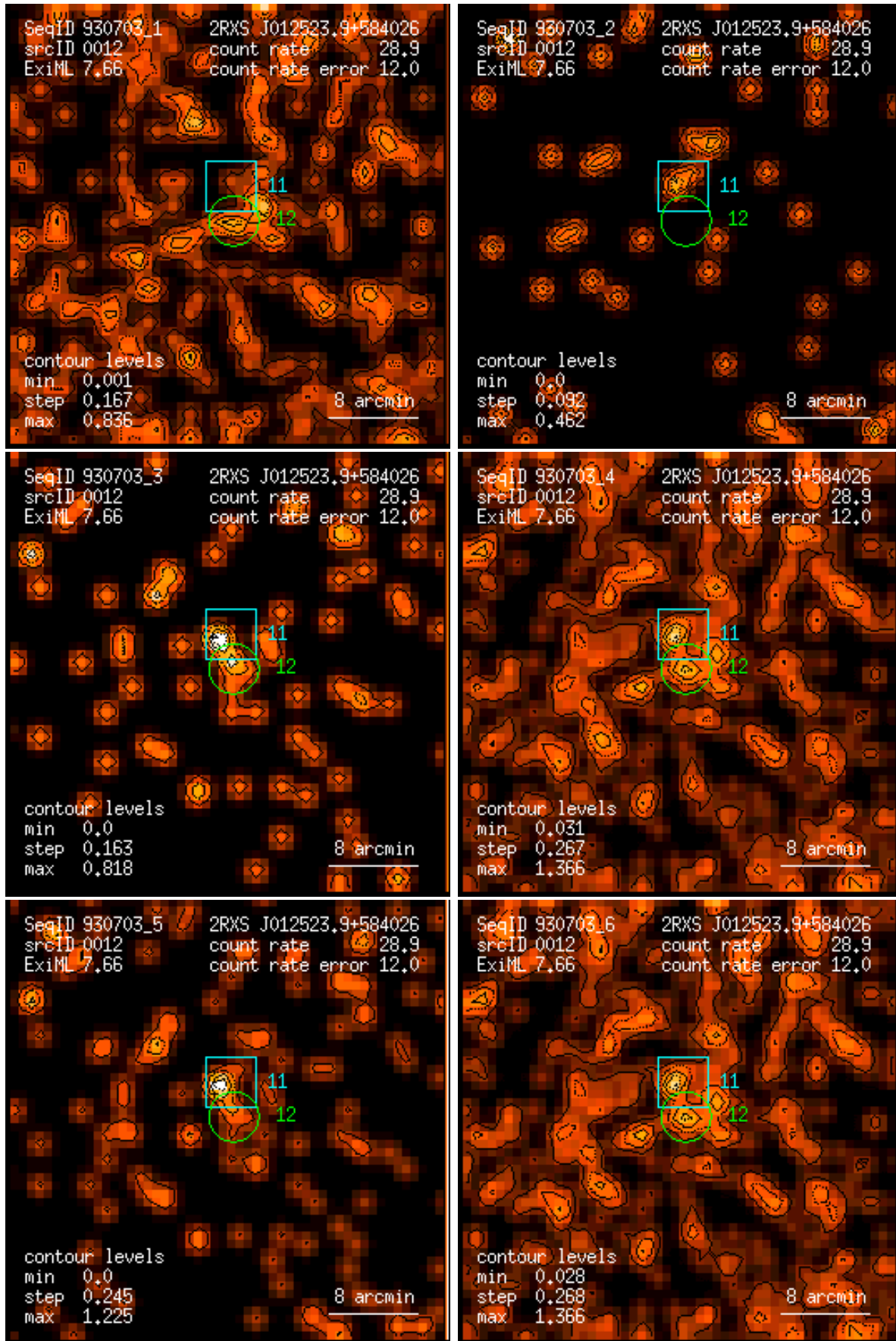
Figure 12: RASS 930703: detection 0012: band rate images, Gaussian filter: (1) PSPC channels 11 – 41, (2) 52 – 90, (3) 91 – 201, (4) 11 – 235, (5) 52 – 201, (6) 11 – 201. Broad band rates in counts/ks. Band rate contour levels in counts/ks/arcmin 2 .
