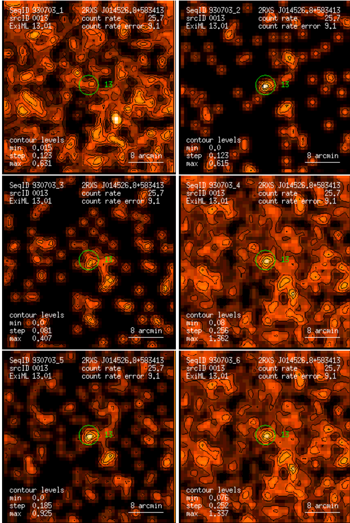
Figure 13: RASS 930703: detection 0013: band rate images, Gaussian filter: (1) PSPC channels 11 – 41, (2) 52 – 90, (3) 91 – 201, (4) 11 – 235, (5) 52 – 201, (6) 11 – 201. Broad band rates in counts/ks. Band rate contour levels in counts/ks/arcmin 2 .
