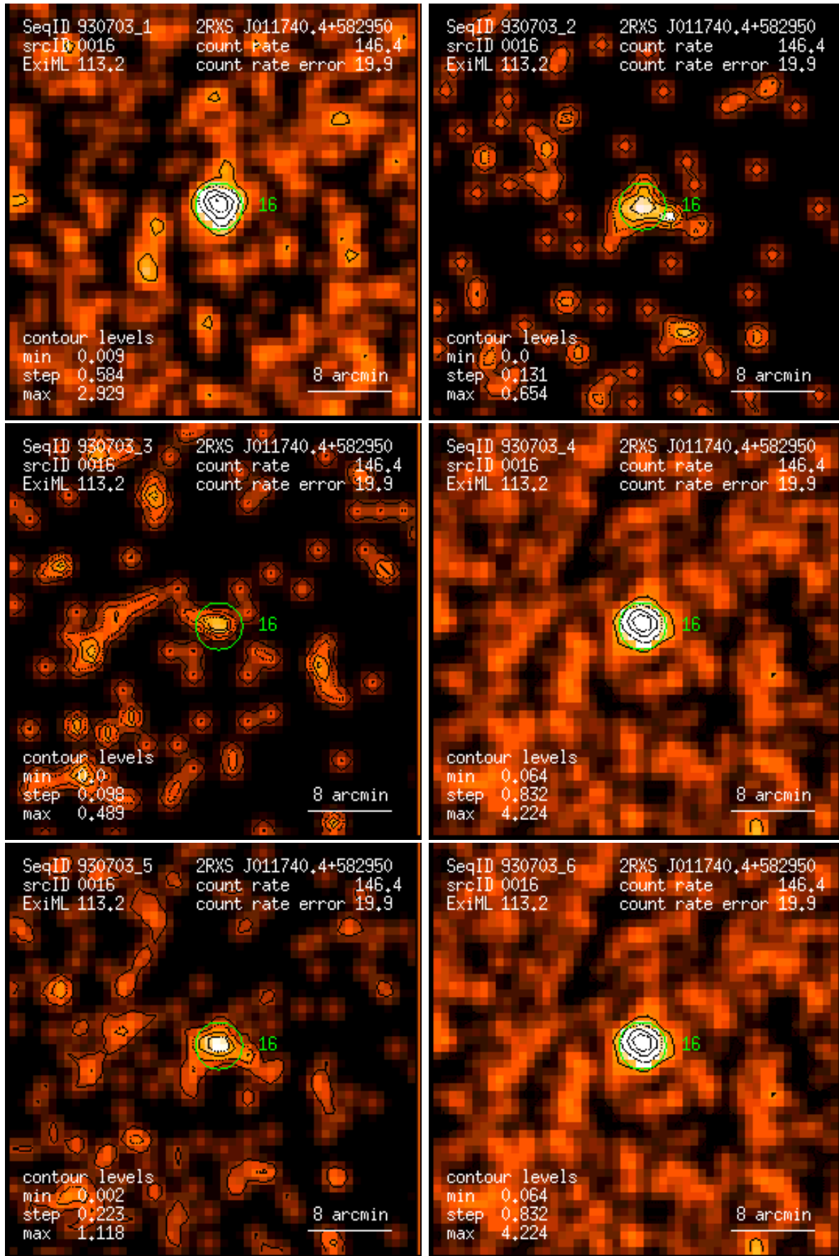
Figure 16: RASS 930703: detection 0016: band rate images, Gaussian filter: (1) PSPC channels 11 – 41, (2) 52 – 90, (3) 91 – 201, (4) 11 – 235, (5) 52 – 201, (6) 11 – 201. Broad band rates in counts/ks. Band rate contour levels in counts/ks/arcmin 2 .
