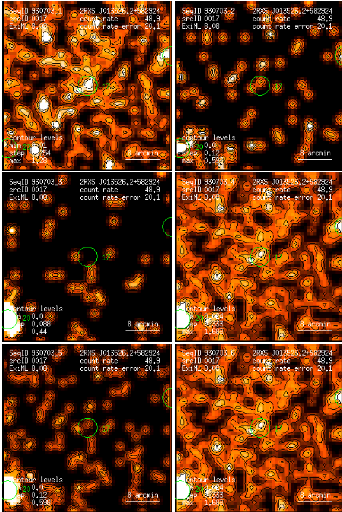
Figure 17: RASS 930703: detection 0017: band rate images, Gaussian filter: (1) PSPC channels 11 – 41, (2) 52 – 90, (3) 91 – 201, (4) 11 – 235, (5) 52 – 201, (6) 11 – 201. Broad band rates in counts/ks. Band rate contour levels in counts/ks/arcmin 2 .
