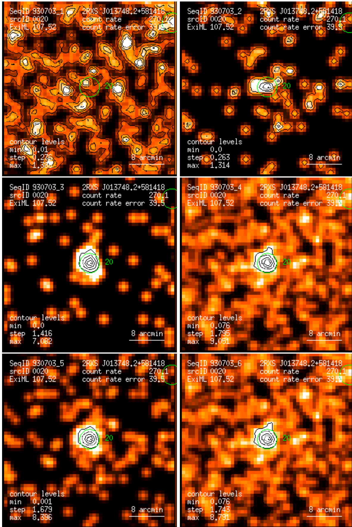
Figure 20: RASS 930703: detection 0020: band rate images, Gaussian filter: (1) PSPC channels 11 – 41, (2) 52 – 90, (3) 91 – 201, (4) 11 – 235, (5) 52 – 201, (6) 11 – 201. Broad band rates in counts/ks. Band rate contour levels in counts/ks/arcmin 2 .
