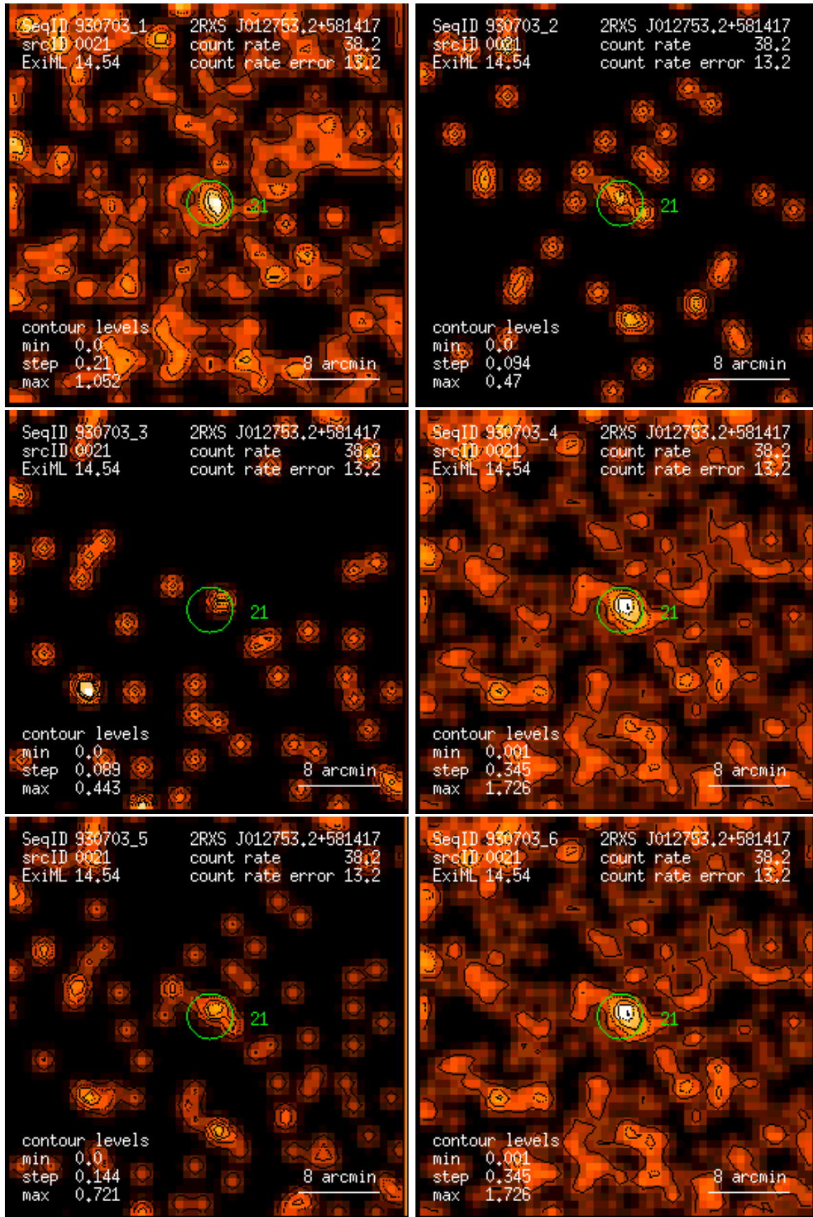
Figure 21: RASS 930703: detection 0021: band rate images, Gaussian filter: (1) PSPC channels 11 – 41, (2) 52 – 90, (3) 91 – 201, (4) 11 – 235, (5) 52 – 201, (6) 11 – 201. Broad band rates in counts/ks. Band rate contour levels in counts/ks/arcmin 2 .
