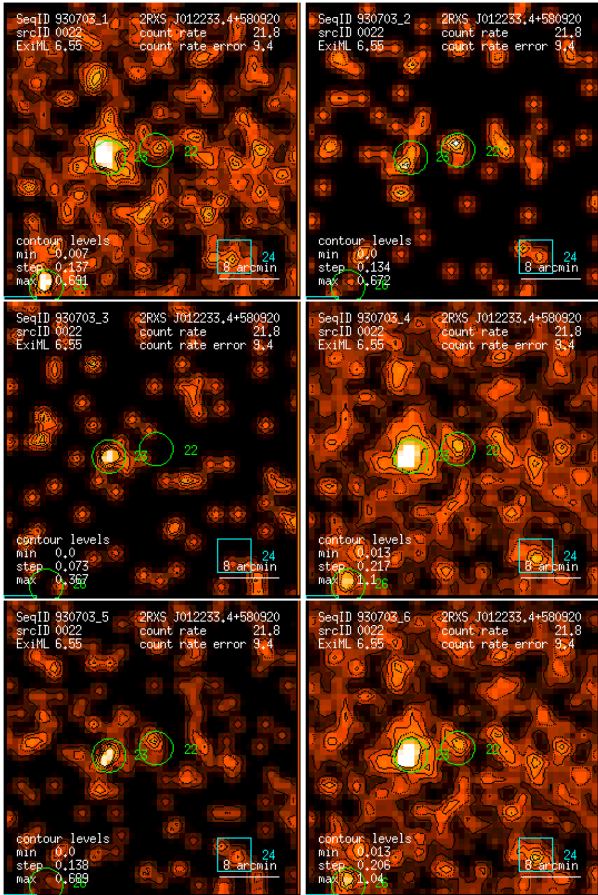
Figure 22: RASS 930703: detection 0022: band rate images, Gaussian filter: (1) PSPC channels 11 – 41, (2) 52 – 90, (3) 91 – 201, (4) 11 – 235, (5) 52 – 201, (6) 11 – 201. Broad band rates in counts/ks. Band rate contour levels in counts/ks/arcmin 2 .
